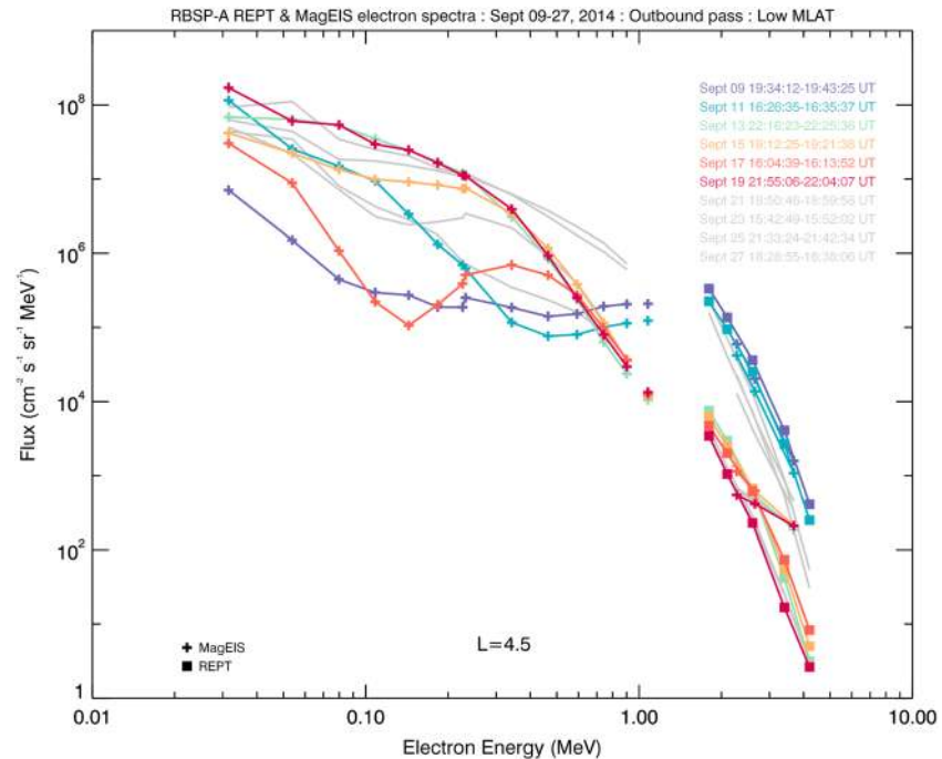
Figure 10. Evolution of energy spectrum across MagEIS and REPT energies: 9–27 September. The gap in the energy spectra from >1 MeV to \sim 2.5 MeV is due to missing MagEIS data channels over this full event period. All spectra are taken from outbound passes at magnetic latitude \leq \sim 5^\circ .
