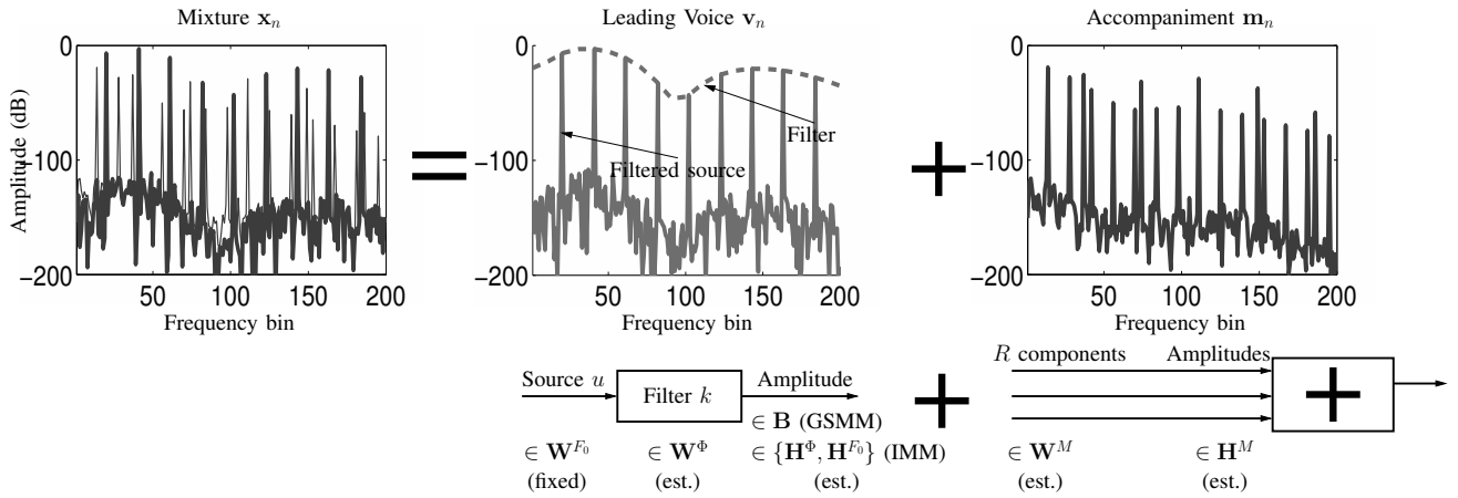
Fig. 2. Principle for the decomposition of one frame of the mixture STFT into leading voice and accompaniment spectra. The parameters indicated here are presented in Section II. The source spectral shapes are fixed as explained in Appendix I and the other parameters are estimated directly from the audio signal.
