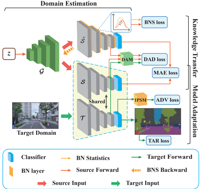
Figure 3. Architecture of the proposed SFDA framework.
