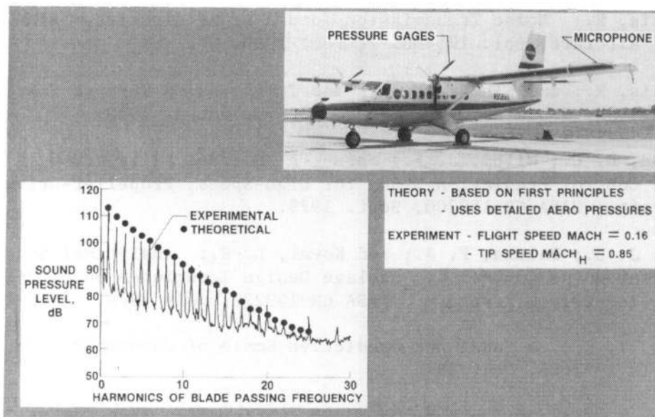
Figure 1.- Measured and predicted noise of general aviation propeller for light, twin-engine transport aircraft.
