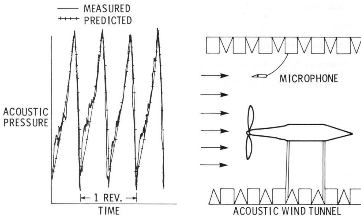
Figure 2.- Measured and predicted noise of low-speed general aviation propeller models.
