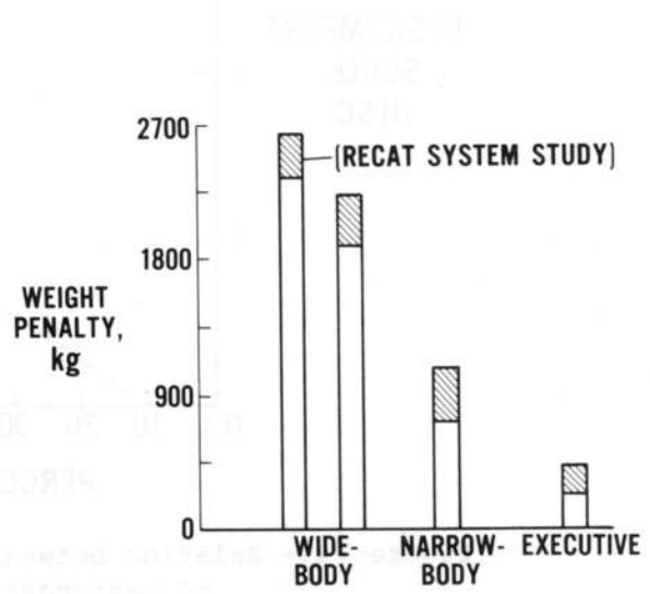
Figure 12.- Theoretical studies of sidewalls for interior noise control on high-speed turboprop aircraft.
