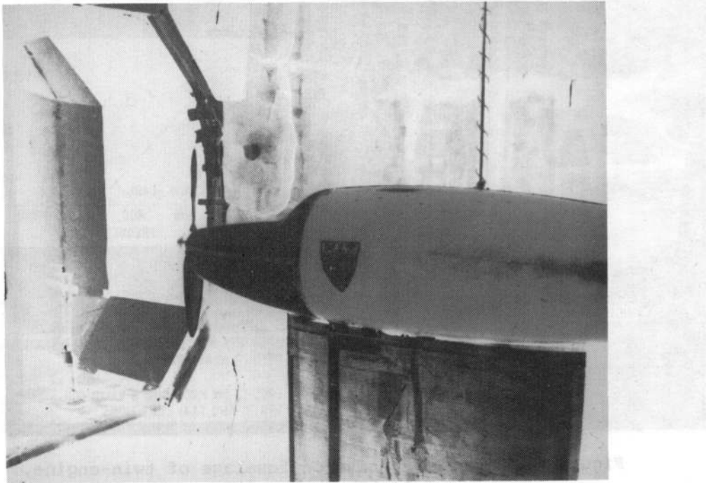
Figure 7.- Acoustic tests of quiet general aviation propellers in anechoic wind tunnel.
