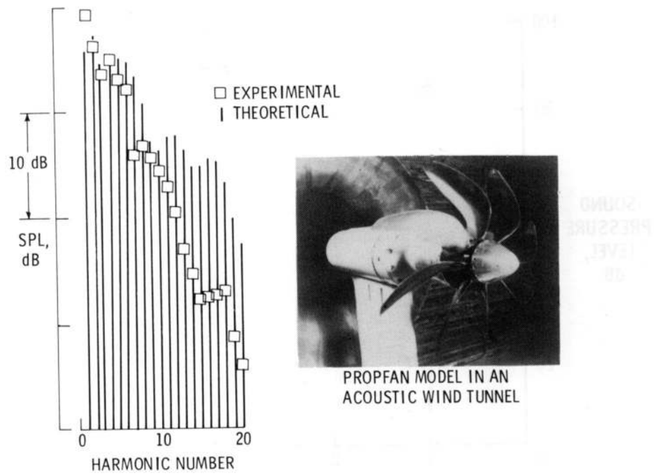
Figure 3.- Harmonic noise spectrum of model high-speed propeller. Diameter = 0.61 m.
