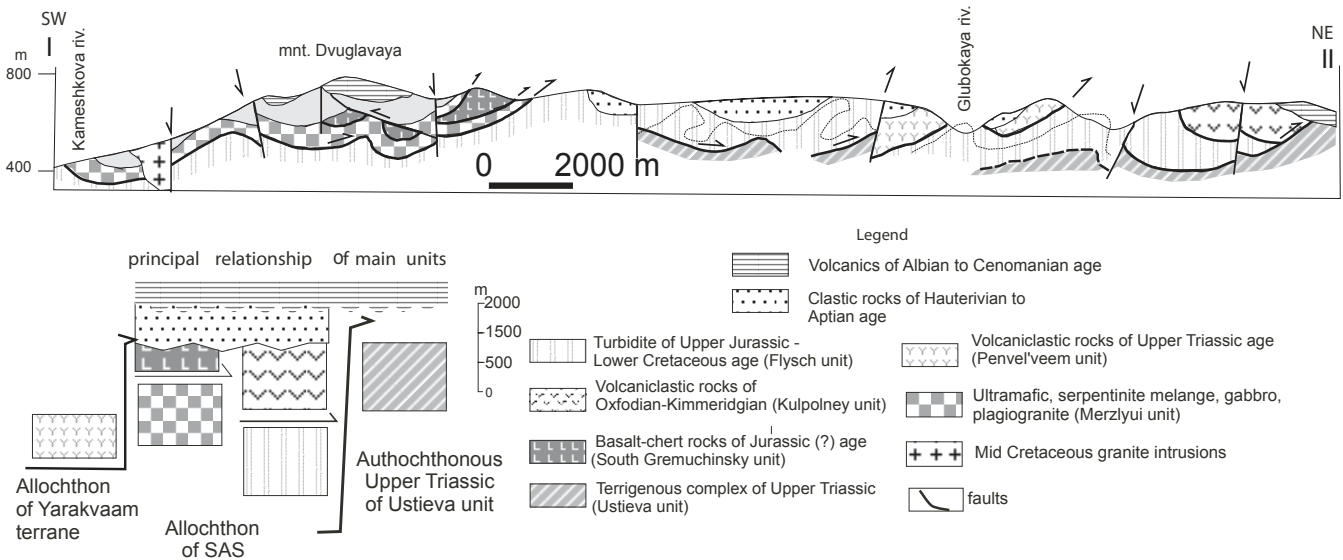
Fig. 10. Geological profile along the line mt. Dvuglavaya-Glubokaya River across the fold-and-thrust structure of SAZ. Place of profile shown on Fig. 3.
