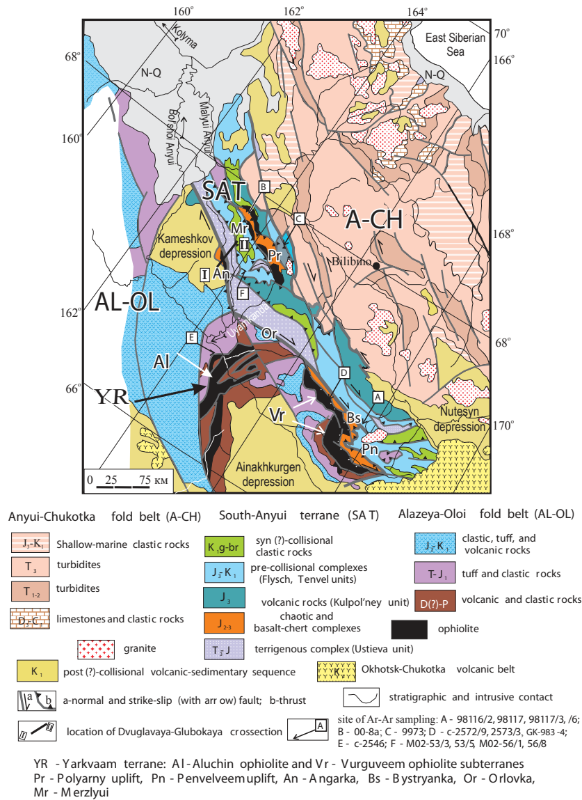
Fig. 3. Tectono-stratigraphic map of Western Chukotka. Compiled by S. D. Sokolov and G. Ye. Bondarenko using their own data and state geological survey maps of 1:200 000 scale (Q-58-III, IV; Q-58-V,VI; Q-58-IX, X; Q-58-XI, XII; Q-58-XV, XVI; Q-58-XVII, XVIII).
