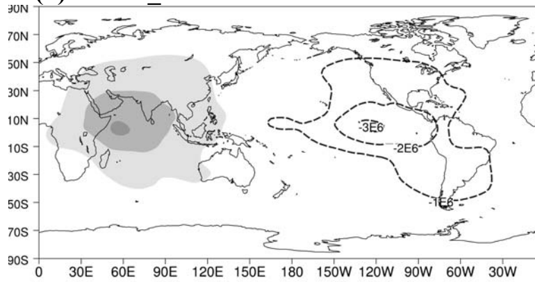
(b) NCAR_PCM
