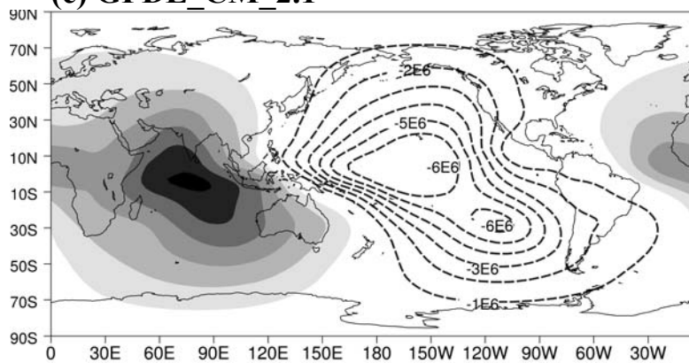
(c) GFDL_CM_2.1
