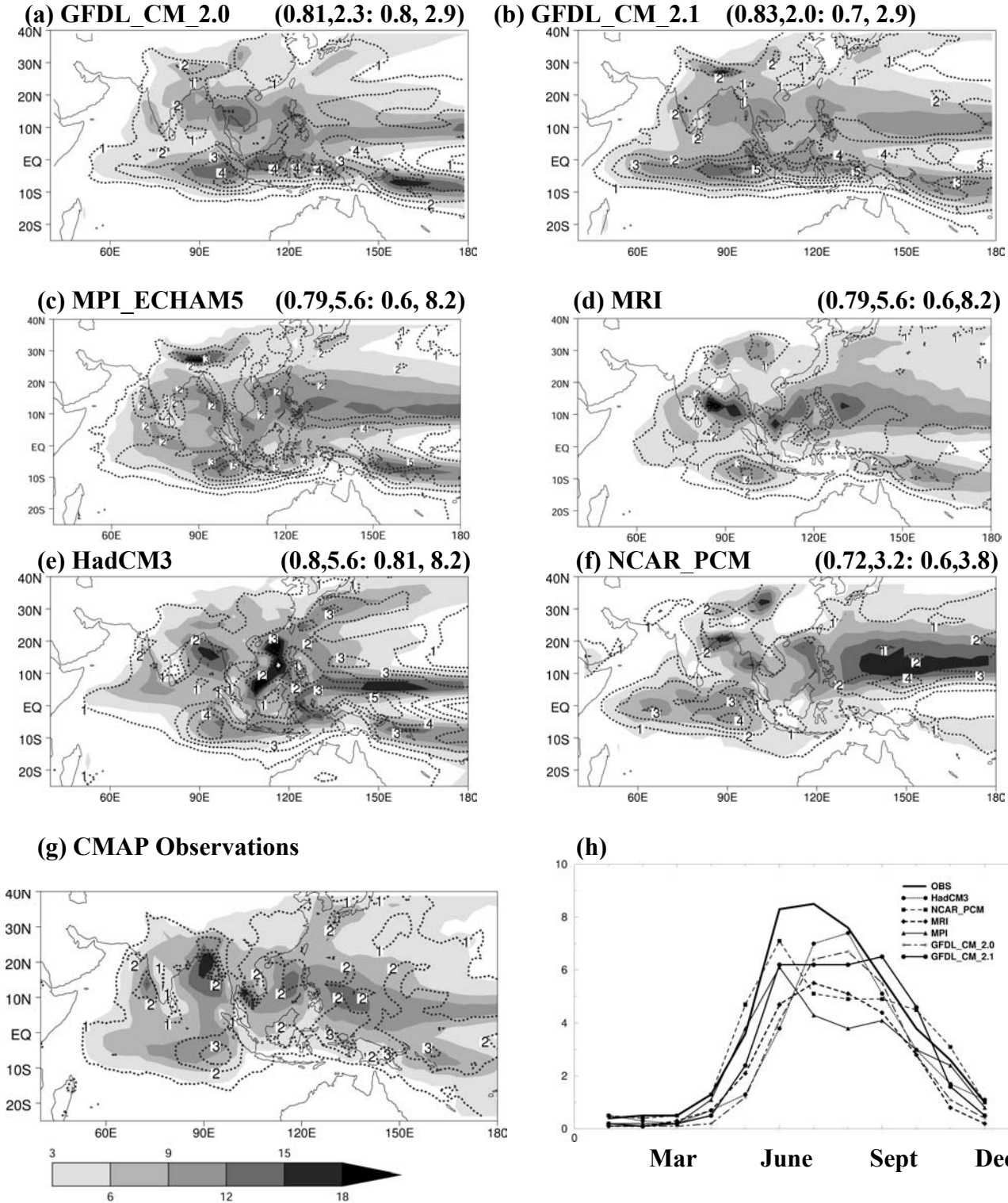
Figure 1: Seasonal mean (June-September) precipitation climatology ( mm/day , shaded) and standard deviation (in dashed contours with an interval of 1.0 \text{ mm/day} ) from the 20c3m integrations of (a) GFDL_CM2.0; (b) GFDL_CM2.1, (c) MPI_ECHAM5, (d) MRI, (e) HadCM3, and (f) NCAR_PCM. Observations are shown in (g). The pattern correlation and the root-mean-square difference (RMSD) between the model and CMAP observations over the Asian Summer Monsoon region ( 40\text{-}180^\circ\text{E} , 25^\circ\text{S}\text{-}40^\circ\text{N} ), and over the Indian monsoon region ( 7\text{-}30^\circ\text{N} , 65\text{-}95^\circ\text{E} ) are given in parenthesis, respectively; (h) annual cycle of precipitation ( mm/day ) over the south Asian monsoon region ( 60\text{-}100^\circ\text{E} , 10\text{-}25^\circ\text{N} ).
