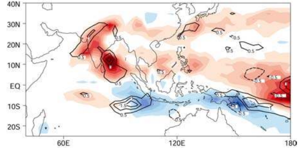
(f) NCAR_PCM
