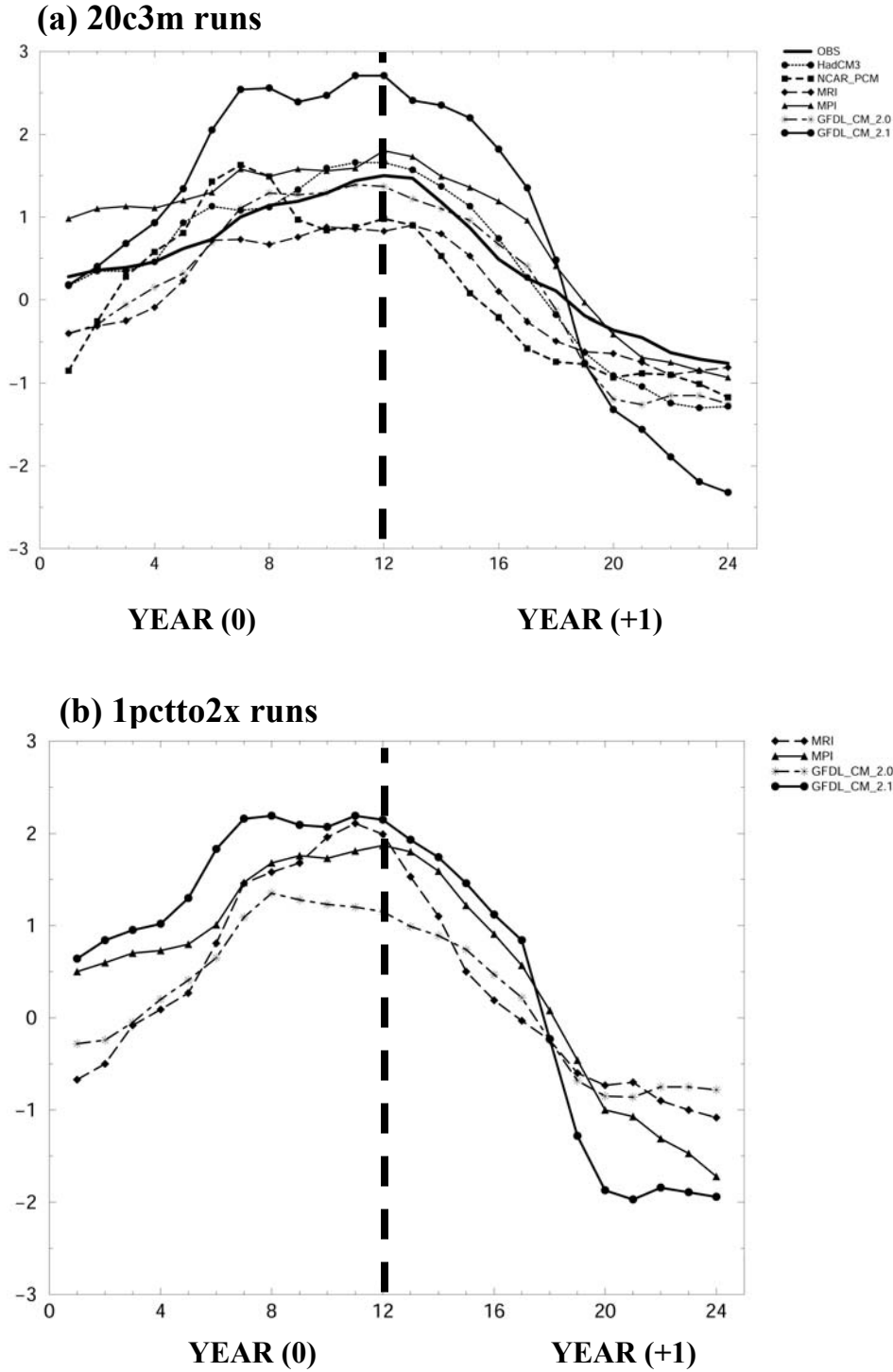
Figure 2: Monthly temporal evolution of composite SST anomalies (in standard deviations) averaged over the NINO3.4 region ( 5^{\circ}\text{S} - 5^{\circ}\text{N} , 120 - 170^{\circ}\text{W} ) from different coupled models: (a) 20c3m and (b) 1pctto2x simulations. The composites are based on strong El Niño events ( > 1.0 std of SST anomalies over the NINO3.4 region). The corresponding figure from observations is also shown in (a). Years 0 and 1 correspond to the typical life cycle of El Niño in which it peaks around December at the end of Year 0.
