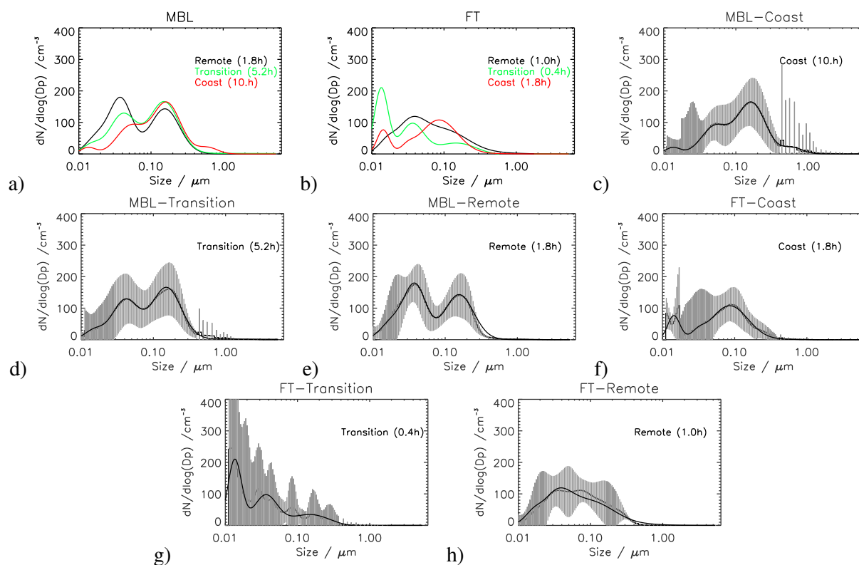
Fig. 12. Particle number size distributions (normalised to natural logarithm of bin width) and log-normal fitted functions between 10 nm and 5 \mu\text{m} in the MBL and FT as labeled, with total sampling time in hours in parentheses: (a) Log-normal fitted functions to median aerosol number spectra for each longitude zone labeled as coloured for the MBL; (b) Log-normal fitted functions for each longitude zone labeled as coloured for the FT; (c) Median MBL coastal zone spectrum (stepped grey line) with corresponding log-normal fit (solid black line); (d) Coastal zone FT spectrum; (e) Transition zone MBL spectrum; (f) Transition zone FT spectrum.; (g) Remote zone MBL spectrum; (h) Remote zone FT spectrum. For each sizing channel, grey bars illustrate one-standard-deviation of the measurement around the median in each channel. Stepped black lines define the median concentration in each sizing channel, whilst the smooth solid black line illustrates the corresponding log-normal fit.
