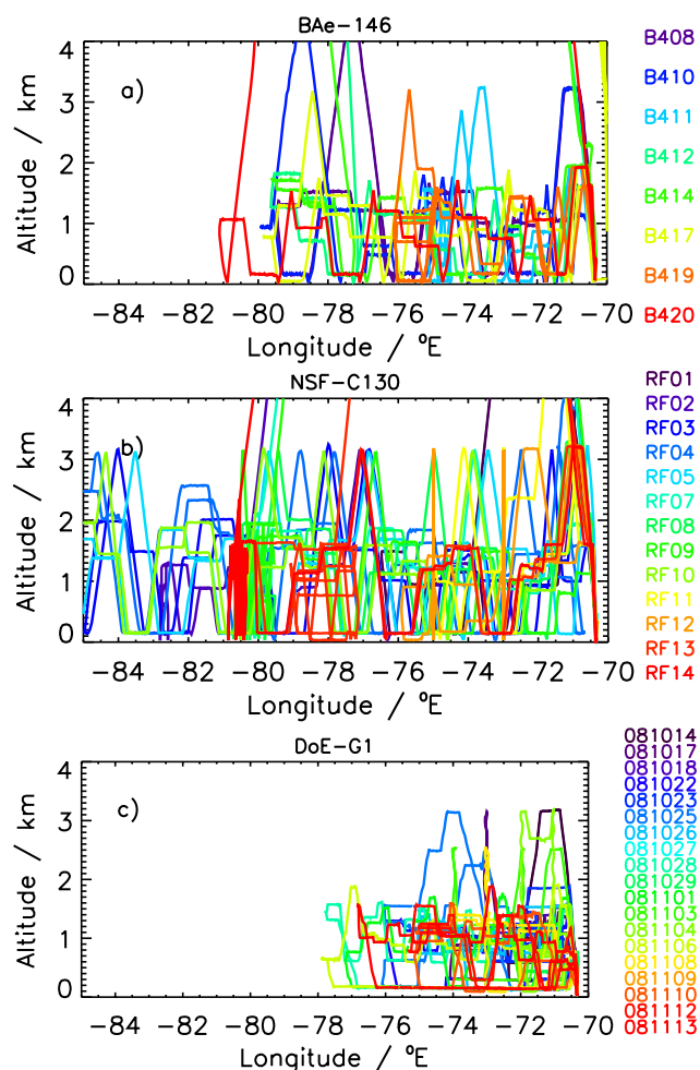
Fig. 1. Flight tracks as longitude-altitude cross-sections of VOCALS-REx flights used in this study and within 1-degree latitude of the 20° South parallel. Individual flight tracks are colour-coded to individual flights to illustrate sampling throughout the course of the VOCALS campaign. Each panel illustrates flight tracks from each of the aircraft platforms as labelled.
