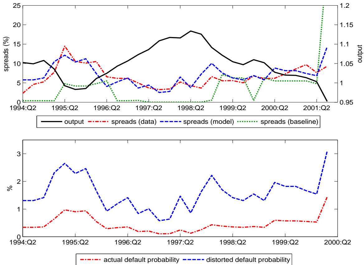
Figure 3: Top Panel: Output for Argentina; spreads generated by our model and the baseline model; and actual spreads (measured by the EMBI+). Bottom Panel: One-step-ahead conditional probabilities of default under the distorted model and the approximating model.
