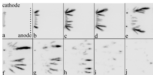
Fig. 2. Light emission evolution across 1.5 cm AK gap at air pressure of 3 \times 10^5 Pa, 1 ns duration HV pulse. Frame duration - 1.5 ns. The time delay of the frame beginning with respect to the appearance of light at the cathode in nanoseconds: (a) 0, (b) 0.3, (c) 1.5, (d) 1.7, (e) 3.1, (f) 4, (g) 6.4, (h) 6.7, (i) 6.9, and (j) 7.8.
