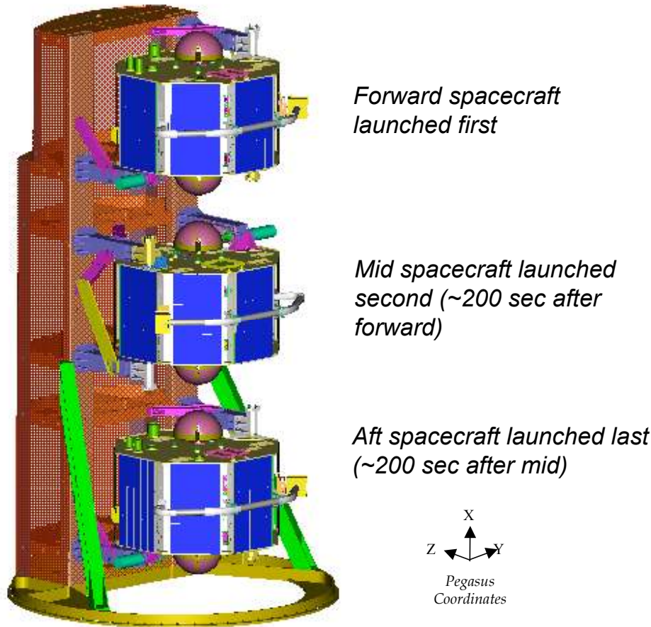
Figure 2— Three ST-5 Spacecraft shown mounted on Pegasus Support Structure. Spacecraft are deployed in the order shown.
