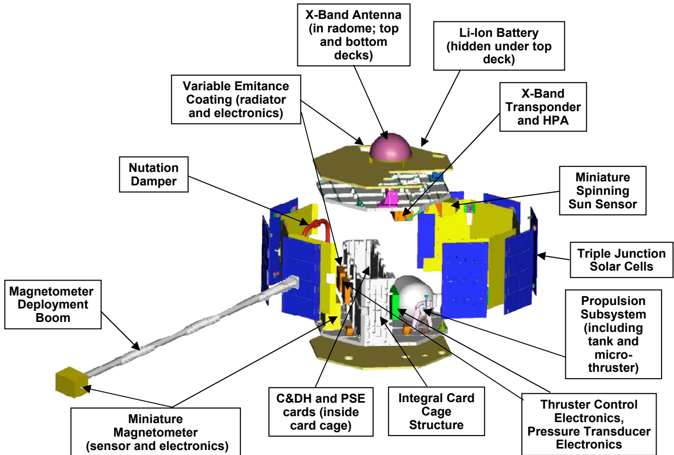
Figure 1— ST-5 Spacecraft Layout. This diagram shows the major components of the ST-5 spacecraft in an "exploded" view.
