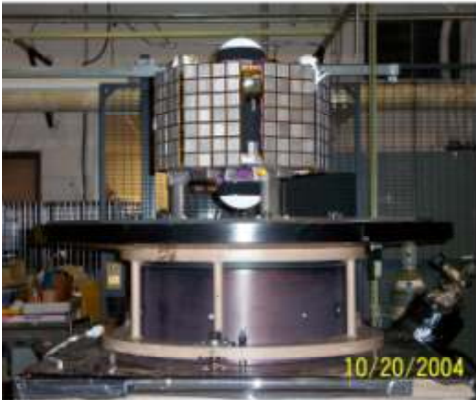
Spacecraft at Mass Properties (shown with solar array mass dummies)
