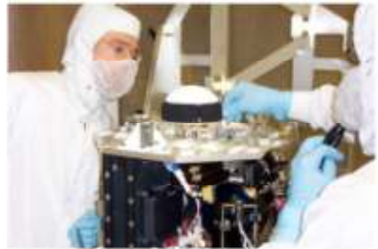
Mounting the Antenna
