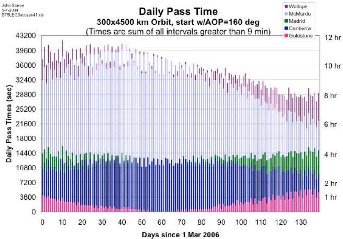
Figure 4 – Ground Station Visibility for ST-5. Because the ST-5 apogee precesses through the southern hemisphere over the 90-day mission, visibility is greatest at southern latitude sites. McMurdo has the best visibility, followed by Canberra.
