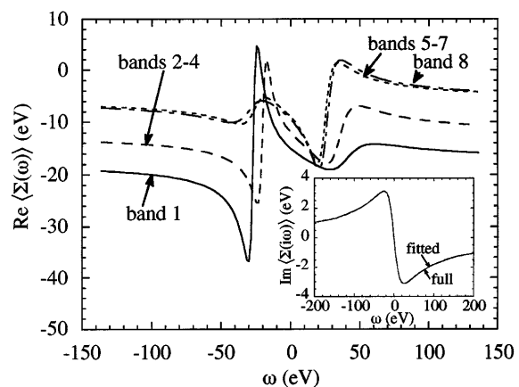
FIG. 2. The matrix element of the self-energy operator of silicon as described onto real energy axis \text{Re}\langle\psi_{n\mathbf{k}}|\Sigma(\omega)|\psi_{n\mathbf{k}}\rangle shown for the first 8 bands at \mathbf{k} = \mathbf{0} . The deviation from a linear function is crucial in obtaining accurate quasiparticle energies away from the band gap (whose center is at zero). Inset: The calculated quantity along the imaginary energy axis \text{Re}\langle\psi_{n\mathbf{k}}|\Sigma(i\omega)|\psi_{n\mathbf{k}}\rangle for band 4 (the valence band maximum), together with the form (6) (with two poles) subsequently used to continue to the real axis; the fit is seen to be excellent.
