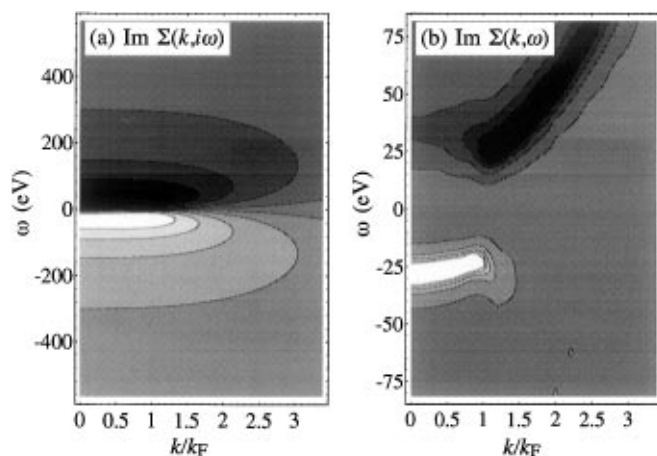
FIG. 1. (a) The GW self-energy of jellium (with density parameter r_s = 2 ) for imaginary energies, calculated using our method [and displayed here as its imaginary part, \text{Im}\Sigma(k, i\omega) ]. (b) The imaginary part of the same quantity analytically continued to the real- \omega axis, \text{Im}\Sigma(k, \omega) . The relative numerical simplicity of (a) is evident, but all relevant information is retained, as shown by (b), which is in excellent agreement with direct calculations. In each plot ten contours are used, from -3 (black) to 3 eV (white) in (a), and from -15 to 15 eV in (b).
