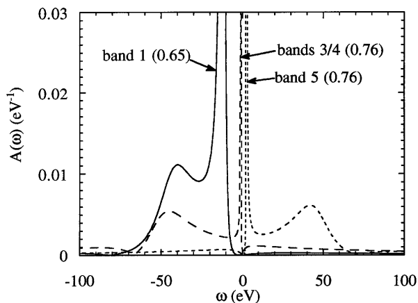
FIG. 3. The spectral function \langle \psi_{nk} | A(\mathbf{r}, \mathbf{r}', \omega) | \psi_{nk} \rangle of silicon, for several bands at \mathbf{k} = (1, 1, 1)\pi/4a . The renormalized quasiparticle poles are evident as sharp peaks, whose calculated weights (the renormalization factors Z ) are given. The spectral background, which includes contributions from plasmons, is also visible.
