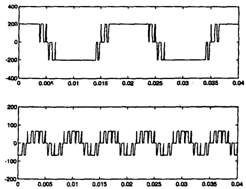
Fig.7b. Motor phase voltage V_{aa'} and 3^{rd} harmonic content- overmodulation
