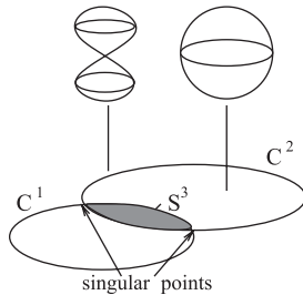
Figure 2: Two curves, C^1 and C^2 , in \mathbb{C}\mathbb{P}^1 \times \mathbb{C}\mathbb{P}^1 with their singular fibration. The shaded region in the base corresponds to an S^3 in the full space.
