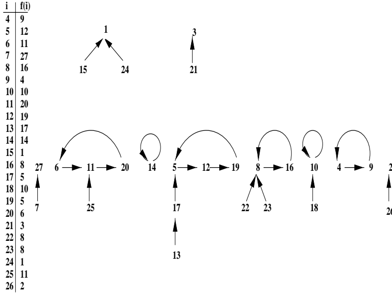
Figure 1: The digraph of a function
