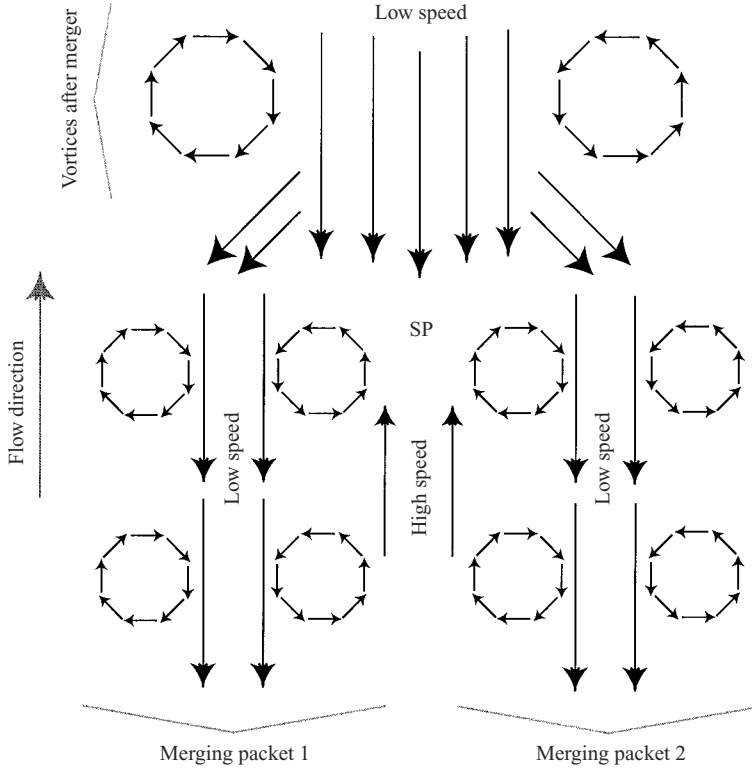
FIGURE 18. Idealized velocity vector signature of merging vortex packets, as viewed in the reference frame of the merging vortices.
