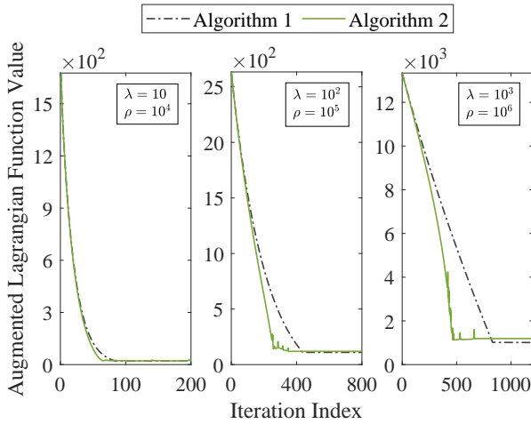
Fig. 2: Function value of \mathcal{L}(\mathbf{w}(k), \mathbf{v}(k), \mathbf{u}(k)) versus iteration index k . (1st example)
