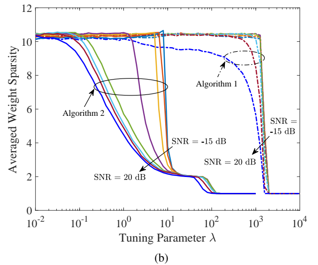
Fig. 3: Sparsity of beamformer weight versus tuning parameter \lambda with (a) INR = 10 dB and (b) INR = 20 dB. (2nd example)
