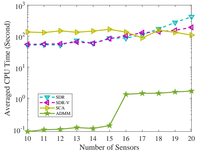
Fig. 5: Averaged CPU time versus M . (4th example)
