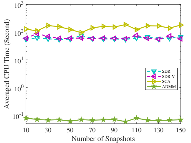
Fig. 4: Averaged CPU time versus T . (3rd example)
