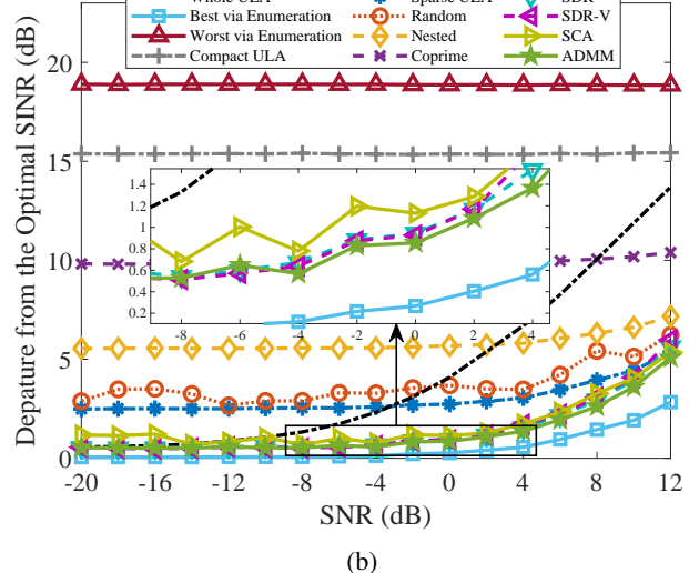
Fig. 9: Output SINR versus input SNR. (8th example)
