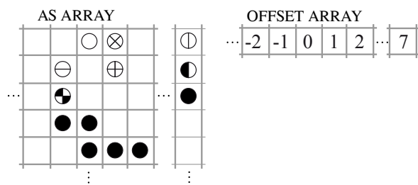
Figure 5: DIA compression of matrix in Figure 1
