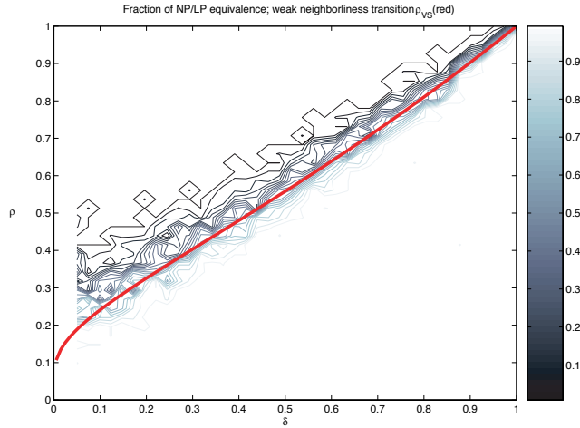
Figure 1: Empirical verification of the NP/LP equivalence phase transition as a function of \delta with d_n = \lfloor \delta n \rfloor and sparsity k = \lfloor \rho d_n \rfloor in the case of n = 200 . The fraction of successes in (LP) recovering (NP) in gray scale, and the calculated weak neighborliness transition curve \rho_{VS}(\delta) overlaid in red. Note that weak neighborliness exceeds d/2 for \delta > .425 ; see Subsection 4.3.
