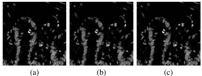
Fig. 9. Restoration of a blur and noisy synthetic image. (a) is the original image, (b) is the degraded version ( PSNR = 28.51 dB), (c) is the result obtained with the Total Variation prior ( PSNR = 32.95 dB), (d) is the result obtained with the proposed prior ( PSNR = 32.02 dB), (e) is the result obtained with the prior proposed in [17] ( PSNR = 31.20 dB).
