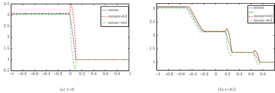
FIGURE 16. Reference solution for the stochastic Euler equations with uncertain initial shock location and amplitude (5.10). We show estimated mean and estimated mean \pm standard deviation.
