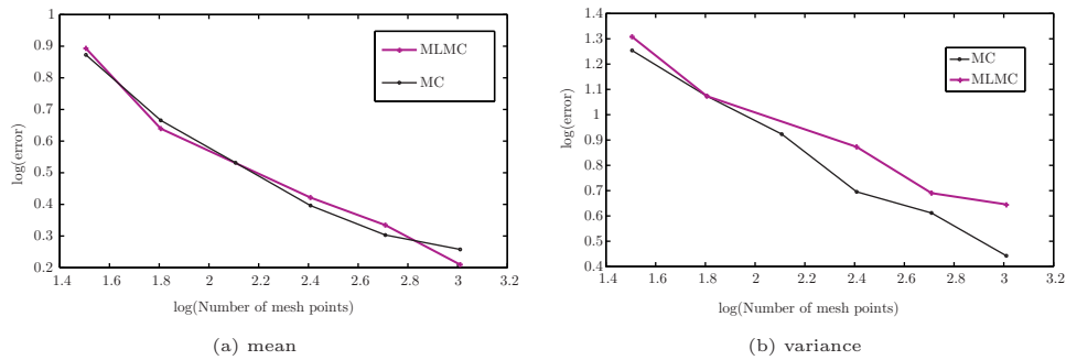
FIGURE 3. A log-log plot for the relative error (y-axis) vs. resolution (x-axis) for the stochastic Burgers' equation (5.1) with uncertain initial amplitude (5.4). MC-FVM and MLMC-FVM are compared.
