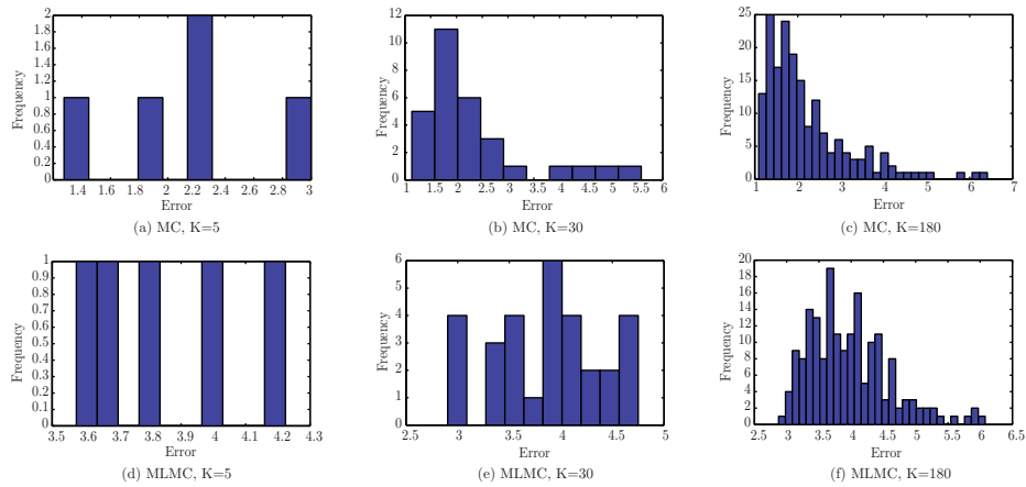
FIGURE 12. Histograms showing the relative error in the mean for each run of the MC and MLMC method for different values of maximum run parameter K = 5, 30, 180 . The mesh resolution is 256 points
