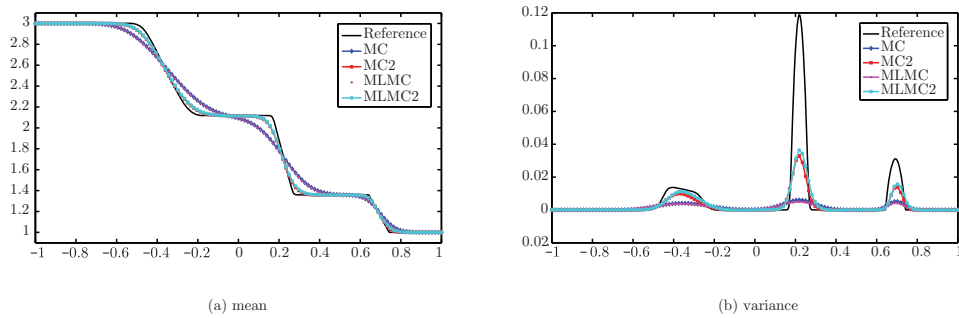
FIGURE 14. Computed solutions for the stochastic Euler equations with uncertain initial shock location (5.9). The graphs depict estimated mean and estimated variance at time t = 0.5 with the MC(2) and MLMC(2) methods.
