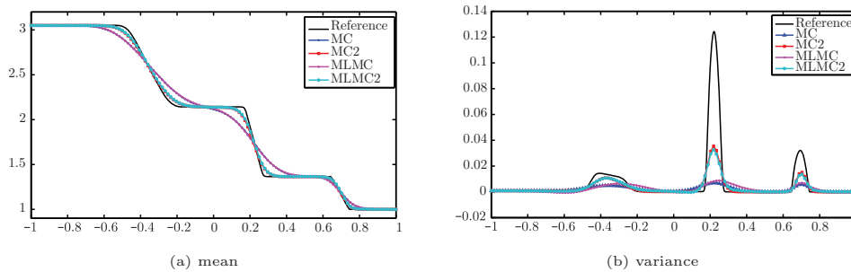
FIGURE 17. Computed solutions for the stochastic Euler equations with uncertain initial shock location and amplitude (5.10). The graphs depict estimated mean and estimated variance at time t = 0.5 with the MC(2) and MLMC(2) methods.
