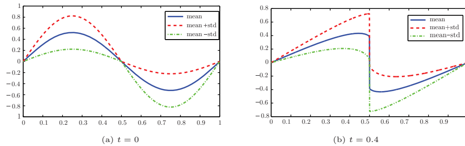
FIGURE 1. Reference solution for the stochastic Burgers' equation (5.1) with uncertain initial amplitude (5.4). The graphs depict estimated mean and estimated mean \pm estimated standard deviation.
