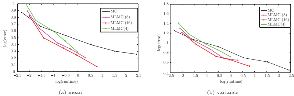
FIGURE 5. A log-log plot for the relative error (y-axis) vs. runtime (x-axis) for the stochastic Burgers' equation (5.1) with uncertain initial amplitude (5.4). The MC-FVM and MLMC-FVMs are compared and the sensitivity of the results to M_L , number of samples at the finest resolution of the MLMC methods is evaluated. We choose M_L = 4, 8, 16 in the above simulations.
