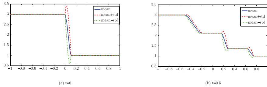
FIGURE 13. Reference solution for the stochastic Euler equations with uncertain initial shock location (5.9). The graphs depict estimated mean and estimated mean \pm standard deviation.
