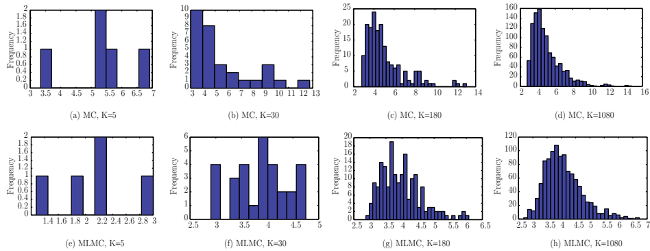
FIGURE 11. Histograms showing the relative error in the mean for each run of the MC and MLMC method for different values of maximum run parameter K = 5, 30, 180, 1080 . The mesh resolution is 64 points
