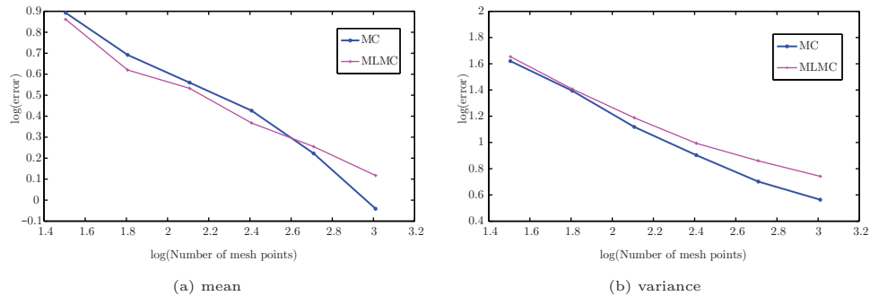
FIGURE 8. A log-log plot for the relative error (y-axis) vs. resolution (x-axis) for the stochastic Burgers' equation (5.1) with uncertain initial phase (5.5). MC-FVM and MLMC-FVM are compared.
