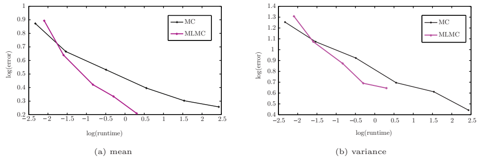
FIGURE 4. A log-log plot for the relative error (y-axis) vs. runtime (x-axis) for the stochastic Burgers' equation (5.1) with uncertain initial amplitude (5.4). MC-FVM and MLMC-FVM are compared.
