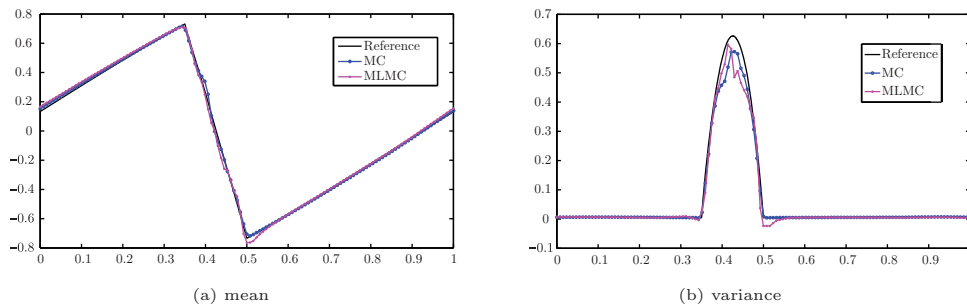
FIGURE 7. Computed solutions for the stochastic Burgers' equation (5.1) with uncertain initial phase (5.5). The graphs depict estimated mean and variance at time t = 0.4 estimated with the MC and MLMC methods, respectively.
