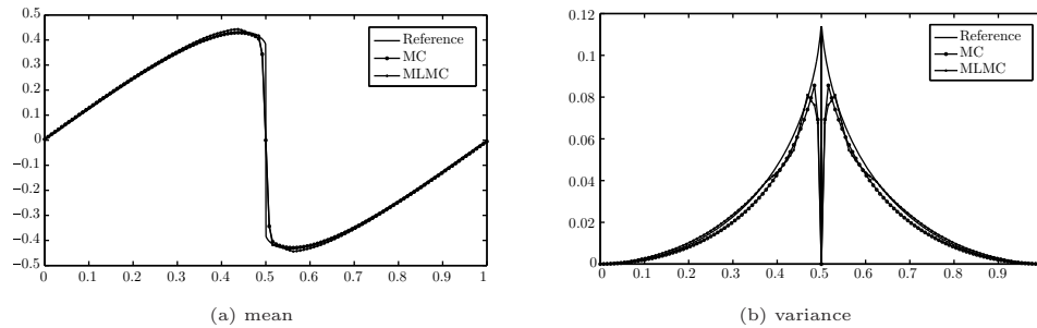
FIGURE 2. Computed solutions for the stochastic Burgers' equation (5.1) with uncertain initial amplitude (5.4). The graphs depict estimated mean and estimated variance at time t = 0.4 computed with the MC-FVM and MLMC-FVM, respectively.
