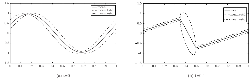
FIGURE 6. Reference solution for the stochastic Burgers' equation (5.1) with uncertain initial phase (5.5). The graphs depict estimated mean and estimated mean \pm estimated standard deviation.
