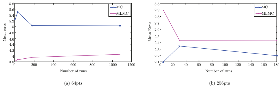
FIGURE 10. The relative mean error vs. maximum run parameter K for the stochastic Burgers' equation (5.1) with uncertain initial phase (5.5). MC-FVM and MLMC-FVM are compared.
