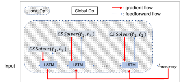
Fig. 2: Sparse-aware training scheme for CSP
