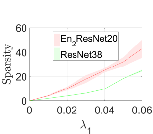
Figure 3: Sparsity of En 2 ResNet20 and ResNet38 under different parameters \lambda_1 . (5 runs)
