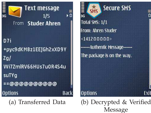
Fig. 7. The data transferred as part of secure SMS and the decrypted message at the receiver.
