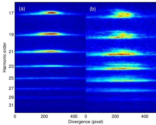
FIG. 8: Harmonic spectra at two different intensities, measured to be 2 \times 10^{14} W/cm 2 (a) and \sim 5 \times 10^{14} W/cm 2 (b). A 21 mm gas cell was used and the focus point of the infrared beam was in the middle of the cell. Note the significant blue shift of the spectral distribution at high intensity.
