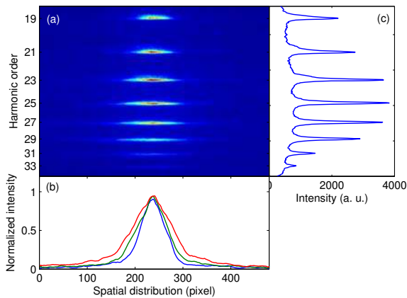
FIG. 4: (a) Experimental measurement using a 21 mm Ar gas cell and a fundamental intensity of I = 10^{14} W/cm 2 ; (b) Spatial profile of the 19 th (blue), 23 rd (green) and 27 th (red) harmonic (c) Spatially integrated spectrum.
