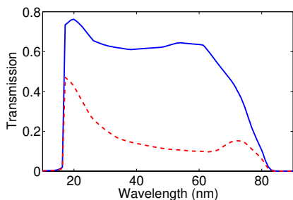
FIG. 6: Calculated transmission function for 200 nm Al filter (blue solid) and with 10 nm oxidation layer on each side (red dashed).
