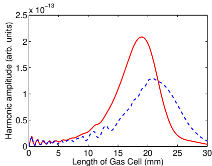
FIG. 2: Phase matching contribution to the harmonic intensity as a function of cell length for short (red solid) and long (blue dashed) trajectories.
