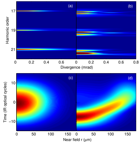
FIG. 9: Calculated far field spatial profile of different harmonic for two different peak intensities, 1 \times 10^{14} W/cm 2 (a) and 3.3 \times 10^{14} W/cm 2 (b). Spatio-temporal distribution of corresponding fundamental beam at the exit of the medium (c) and (d).
