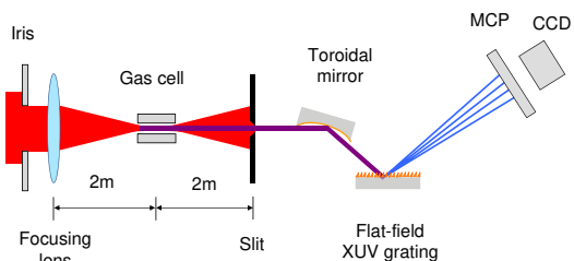
FIG. 3: Experimental setup.
