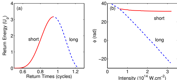
FIG. 1: (a) Classical calculation of the kinetic energy of the electron as a function of the return time. (b) Calculation of the intensity dependence of the 19 th harmonic phase for the short and long trajectories using the strong field approximation [19].
