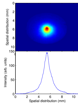
FIG. 5: Spatial profile of the total harmonic yield transmitted through the Al filter measured at 2 m from the 15 mm gas cell. The infrared beam was focused just at the beginning of the cell. The aperture was 14 mm.
