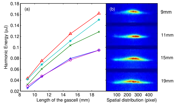
FIG. 7: (a) Harmonic energy as a function of cell length for the 13^{th} (line with plus), 17^{th} (line with x-mark), 21^{st} (line with triangle), 23^{rd} (line with star) and 27^{th} (line with circle) order. (b) Spatial distribution of 23^{rd} harmonic for different gas cell lengths.
