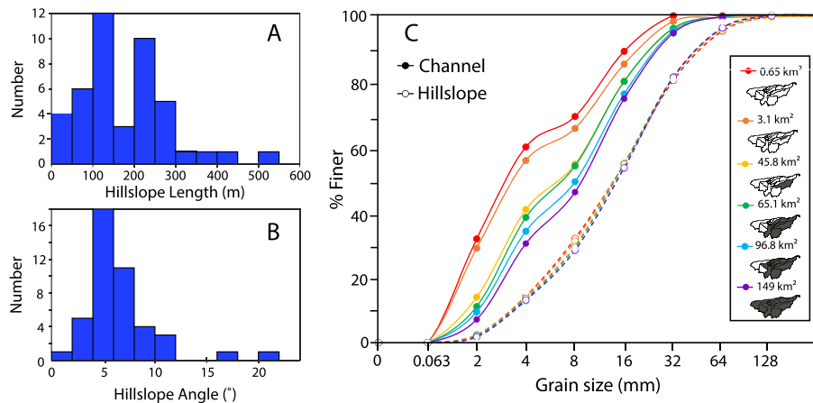
Figure 5. Field data: histograms of hillslope lengths (A) and angles (B) measured in Walnut Gulch Experimental Watershed (WGEW), and the aggregated grain-size distributions (GSDs) downstream for all channel locations (solid line with filled symbols) and hillslopes (dashed lines with open symbols) within each colour-coded nested watershed area (C). [Colour figure can be viewed at wileyonlinelibrary.com ]
