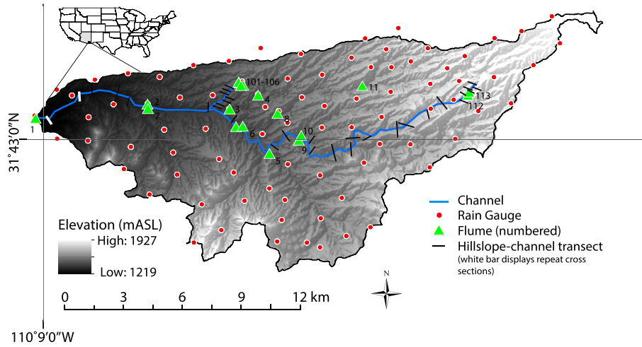
Figure 1. Walnut Gulch Experimental Watershed near Tombstone, Arizona, USA showing locations of hillslope–channel transects, rain gauges and channel flumes. Base map data source: US Geological Survey (USGS) 10 m digital elevation model (DEM). [Colour figure can be viewed at wileyonlinelibrary.com ]
