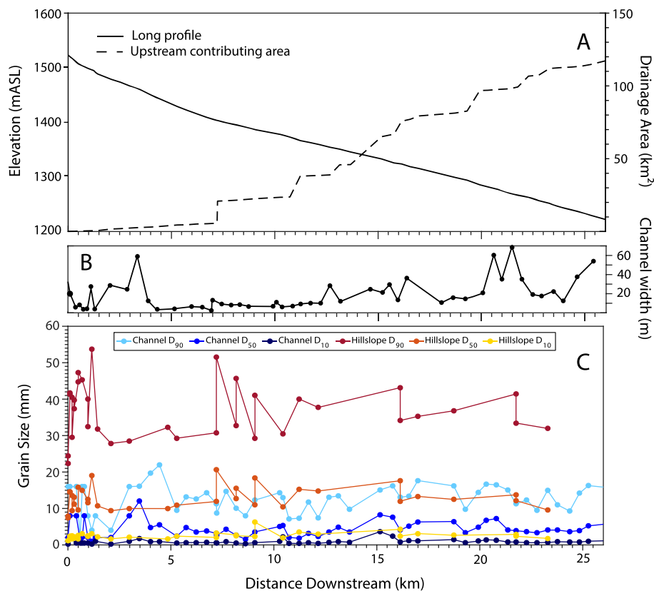
Figure 4. (A) Longitudinal profile and corresponding drainage area, (B) channel width and (C) characteristic grain sizes on hillslopes and in the channel. There is a statistical similarity between hillslope D_{50} and channel D_{90} (Kolmogorov–Smirnov statistic = 0.18, p = 0.28 , n_1/n_2 = 72/31 ). [Colour figure can be viewed at wileyonlinelibrary.com ]
