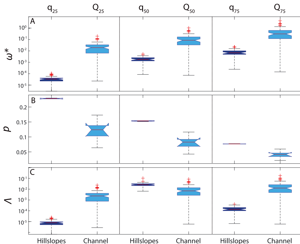
Figure 7. Box and whisker plots displaying the median and interquartile range for dimensionless stream power, \omega^* (A), probability of occurrence, p (B) and their product \Lambda (C) at each percentile of flow used in this study. Data are grouped by hillslopes and channels. [Colour figure can be viewed at wileyonlinelibrary.com ]
