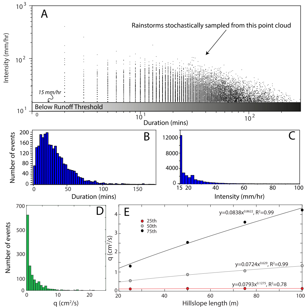
Figure 3. (A) Phase space of rainfall intensity versus duration. These data were thresholded at 15 mm/h, for all data measured at Walnut Gulch Experimental Watershed (WGEW) since 1953 (black dots). We sampled from this distribution and then used these data to drive COUP2D. (B) Histogram of all rainfall durations for storm events > 15 mm/h and the quartile values for the distribution. (C) Histogram of rainfall intensities for rainfall events > 15 mm/h and the extracted intensities for each curve in (A). (D) Histogram of all modelled hillslope runoff ( n = 1832 ), based on stochastic simulation of runoff on slopes of four different lengths. (E) Relationships between hillslope length and the q percentiles of modelled runoff used later to calculate the q percentiles for the measured hillslopes in WGEW. [Colour figure can be viewed at wileyonlinelibrary.com ]
