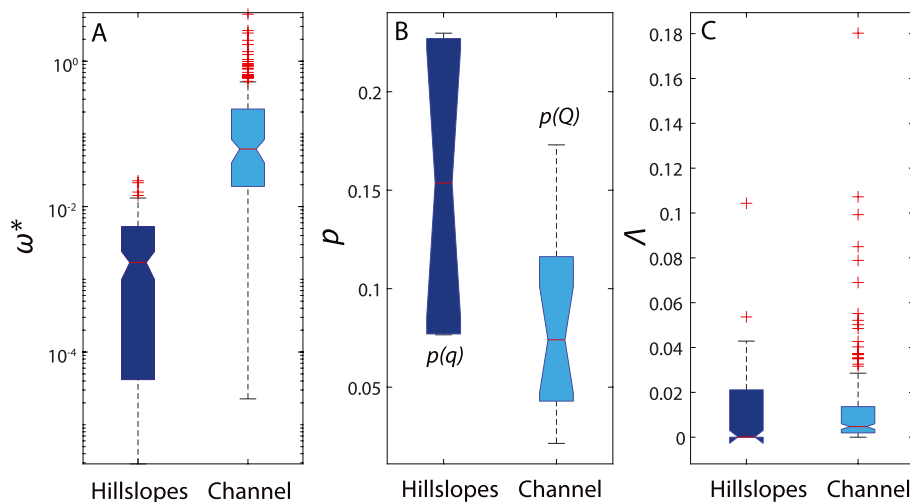
Figure 6. (A) Box and whisker plots displaying the median and interquartile range of dimensionless stream power, \omega^* . (B) Probability of occurrence, p . (C) The product of dimensionless stream power and the probability of occurrence, \Lambda , for hillslopes and channel locations in Walnut Gulch Experimental Watershed (WGEW). [Colour figure can be viewed at wileyonlinelibrary.com ]
