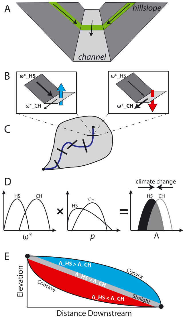
Figure 10. A schematic of the framework set out in this study. At hillslope–channel transects (A) we assess the net balance of \omega^* as a proxy for sediment transport (B). If the stream power in the channel is greater than the stream power on the hillslope, then the channel bed will degrade, and vice versa. We assess the net balance at transects throughout the basin (C). Our framework includes the calculation of \omega^* , the frequency of corresponding flows, p , and the product of these, \lambda , to assemble pdfs of net balance over a multi-decadal time period (D). When the net balance, between \lambda_{\text{HS}} and \lambda_{\text{CH}} is positive, the longitudinal profile will tend toward convex up and vice versa (E). In drylands, however, straight profiles are often observed, suggesting zero N_{\text{Bal}} . Climate changes that differentially alter runoff regimes on slopes and in the channel, can change this balance. At Walnut Gulch, lower rainfall intensity favouring more storms would shift lambda distributions closer together (D), reinforcing a zero N_{\text{Bal}} . [Colour figure can be viewed at wileyonlinelibrary.com ]
