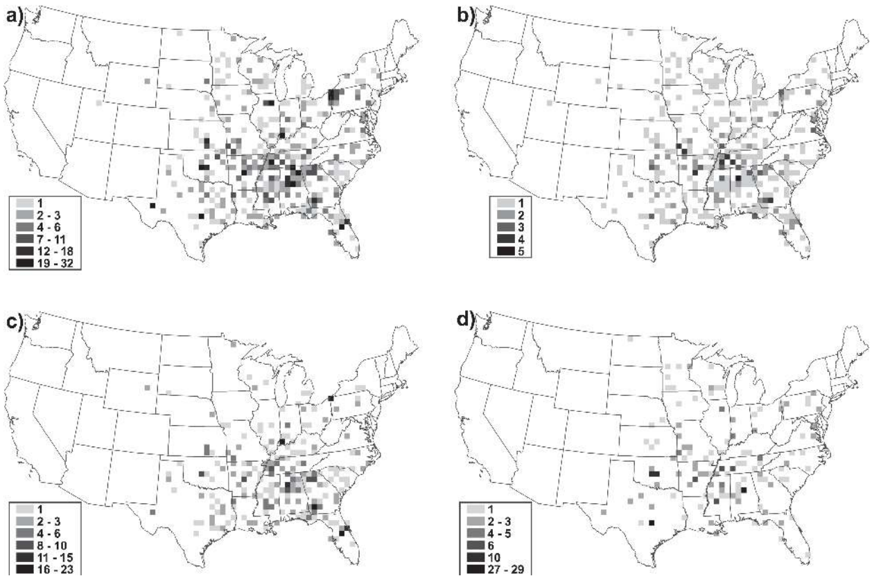
FIG. 7. Number of (a) tornado fatalities, (b) killer tornado events, (c) mobile home fatalities, and (d) permanent home fatalities in a 60 \text{ km} \times 60 \text{ km} grid for 1985–2005.
