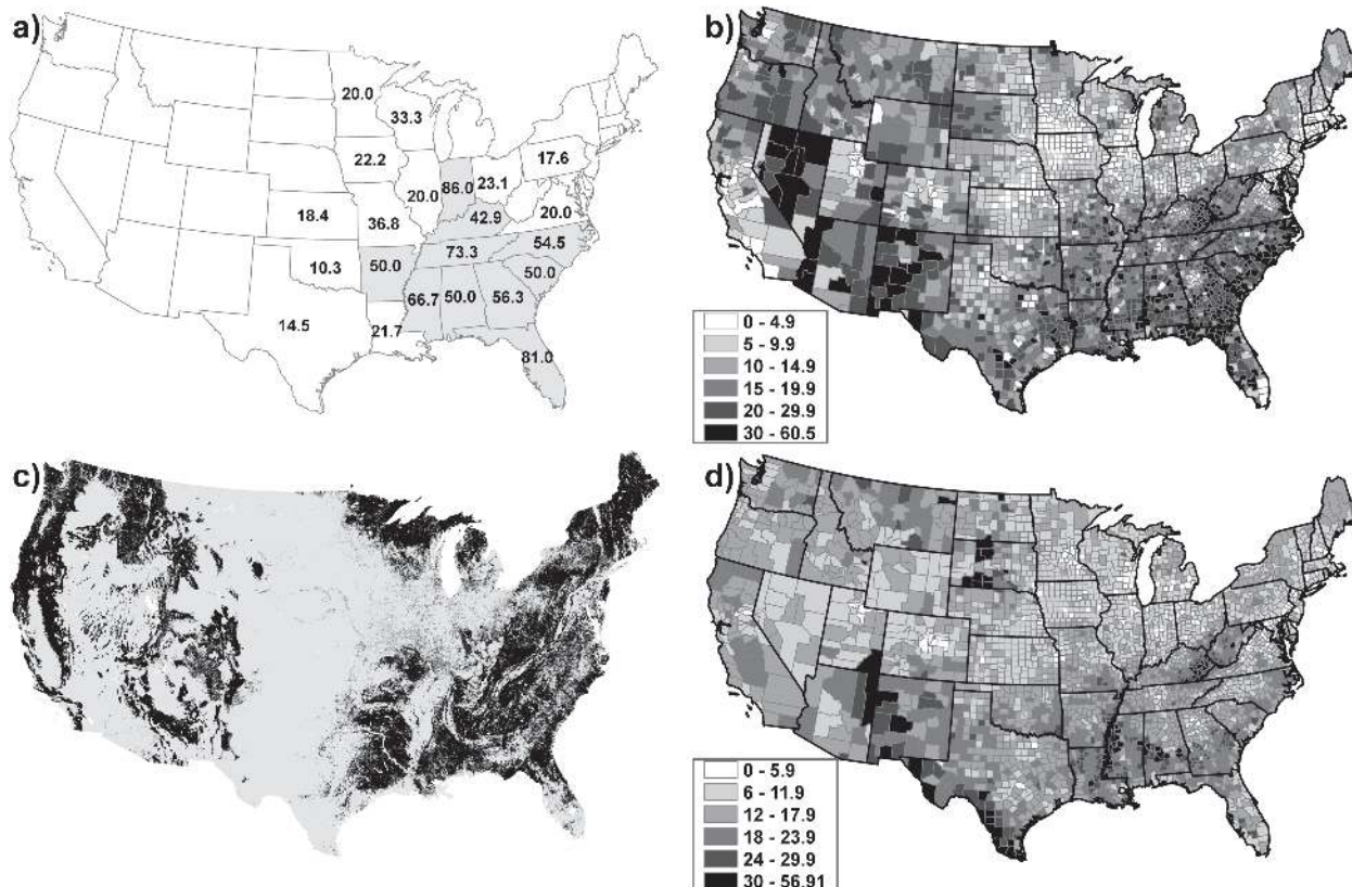
FIG. 8. (a) Percentage of nighttime tornado fatalities by state (illustrated for those states with greater than 10 tornado fatalities for 1985–2005; shaded states above the national average for nighttime tornado fatalities of 42.5%), (b) percentage of mobile homes by county (U.S. Census Bureau 2006), (c) forest cover (solid black) for the United States as determined by Advanced Very High Resolution Radiometer data (information online at http://nationalatlas.gov/articles/biology/a_forest.html ), and (d) percent of county population in poverty (U.S. Census Bureau 2006).
