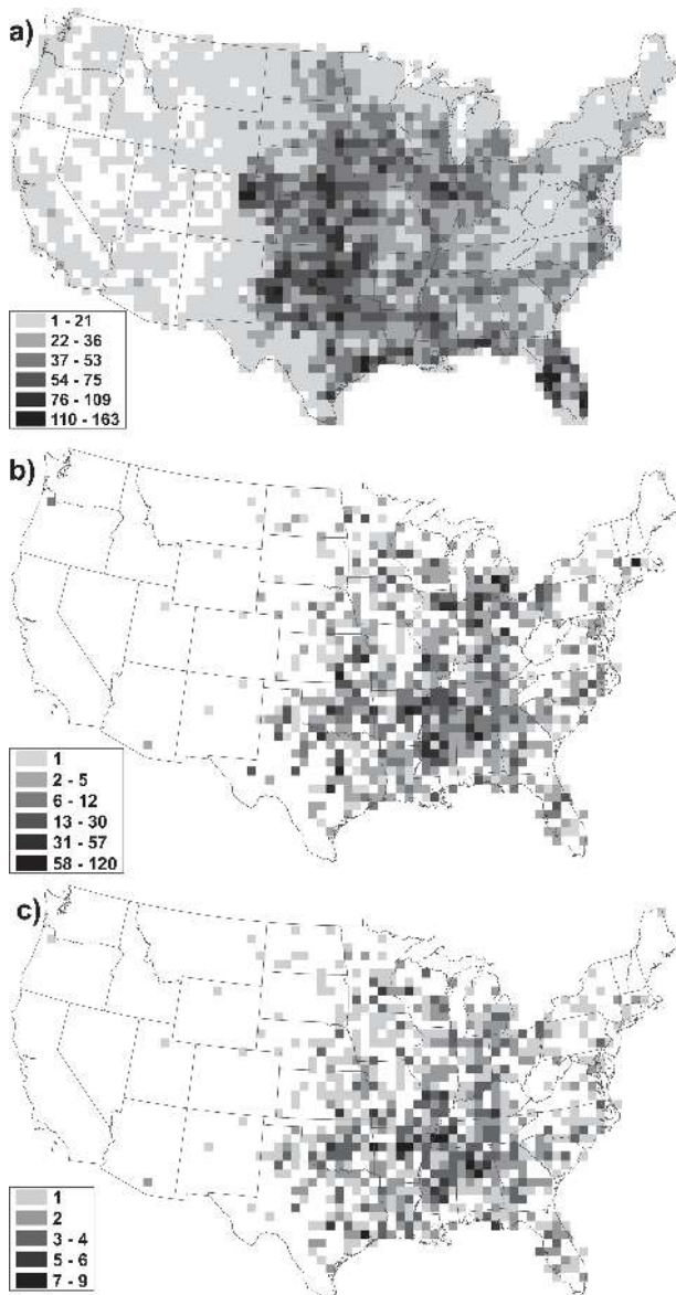
FIG. 5. Number of (a) tornadoes, (b) tornado fatalities, and (c) killer tornado events in a 60 km \times 60 km grid for 1950–2004.
