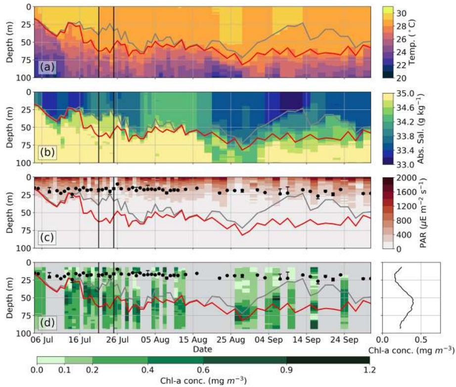
Figure 6. Time series of observations measured by float 631, linearly interpolated to 1 m depth intervals: (a) temperature (°C), (b) absolute salinity (g kg -1 ), (c) PAR μE m -2 s -1 , and (d) chlorophyll concentration with the vertical profile of the average chlorophyll concentration (mg m -3 ). Grey sections in the chlorophyll time series represent removed E d (490) profiles that displayed excessive noise. The black dots are scale depth values, h 2 (m). The region between the MLD (grey line) and isothermal layer depth (red line) is the barrier layer.
