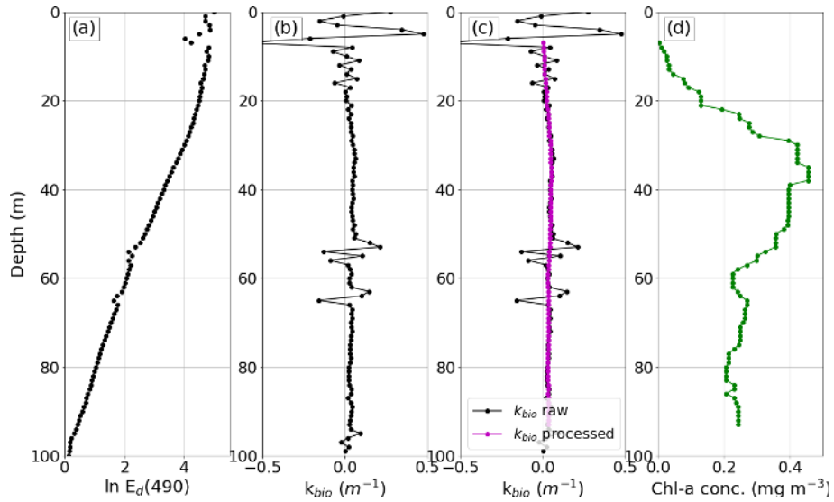
Figure A1. (a) Profile of \ln E_d(490) from dive 10, float 631, interpolated onto a 1 m vertical grid. (b) The attenuation due to biological constituents, K_{bio} (m^{-1}) . (c) K_{bio} (m^{-1}) before quality control processing (black dotted line) and after quality control processing (magenta dotted line). (d) Chlorophyll a concentration ( mg m^{-3} ) (green dotted line).
