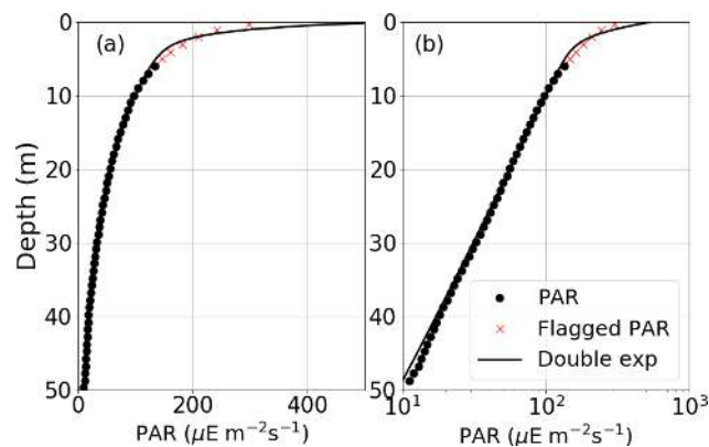
Figure 2. (a) Profile of PAR (black circles) measured from float 629 from the surface to 50 m of depth with a fitted double exponential function (black line) to PAR between 5 and 100 m of depth. R and h_1 were specified to be 0.67 and 1.0 m, respectively. Red crosses show flagged PAR values that were excluded from the curve fit. (b) Same vertical profile of PAR and fitted double exponential function as (a), but presented in log space.
