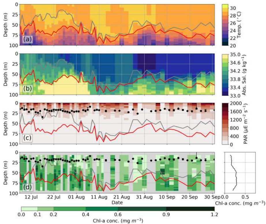
Figure 8. As Fig. 6 but for float 630.
