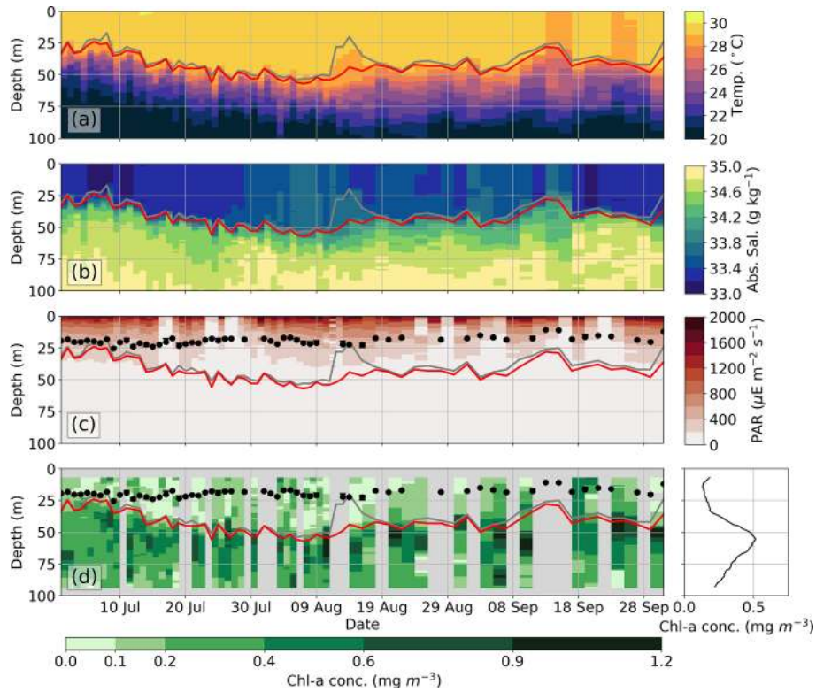
Figure 7. As Fig. 6 but for float 629.
