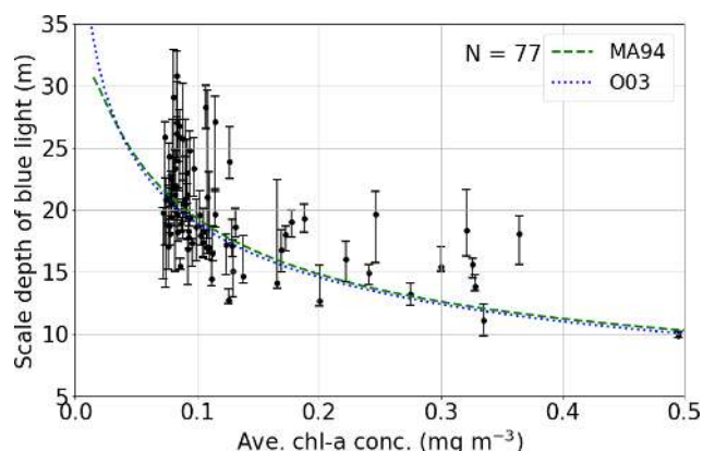
Figure 9. Observed h_2 against average chlorophyll a concentration between the surface and 30 m of depth from glider SG579 (black circles). Parameterizations of the scale depth of blue light (equivalent to h_2 ) for chlorophyll concentrations between 0 and 0.5 \text{ mg m}^{-3} are presented with the observational data: Morel and Antoine (1994) (MA94) (dashed green line) and Ohlmann (2003) (O03) (dotted blue line).
