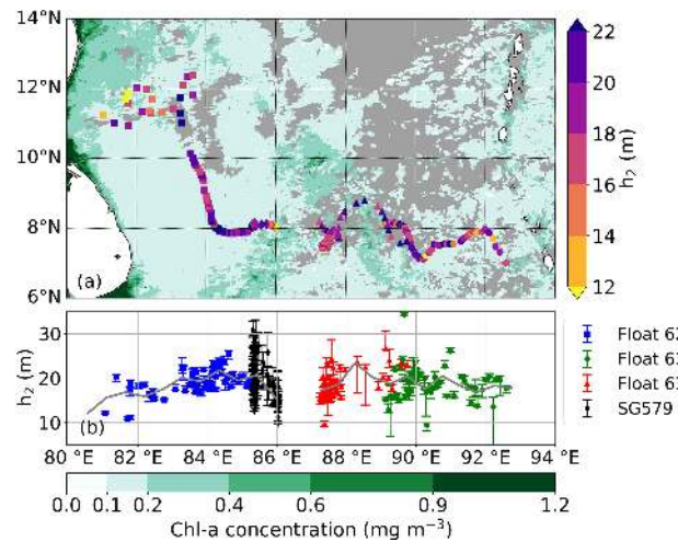
Figure 5. (a) Location of each profile for glider SG579 (diamond), float 629 (square), float 630 (circle), and float 631 (triangle) across the southern Bay of Bengal coloured by the observed h_2 value. The ESA OC-CCI version 3.1 satellite composite of 4 km chlorophyll a concentration for the month of July 2016 is shown. (b) The h_2 variability with longitude across the basin for glider SG579 (black diamond), float 629 (blue square), float 630 (green circle), and float 631 (red triangle). The grey solid line represents the mean h_2 value binned at 0.5^\circ intervals.
