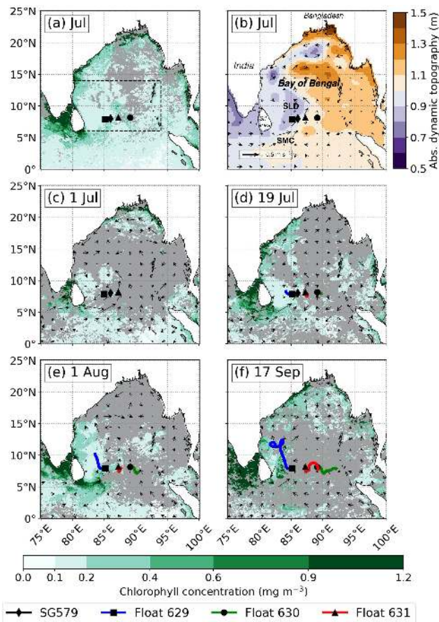
Figure 1. (a) Satellite composite of July 2016 average 4 km chlorophyll a concentration ( \text{mg m}^{-3} ) obtained from ESA OC-CCI version 3.1. The dashed black box shows the outline of Fig. 5a. (b) Absolute dynamic topography (m) of horizontal resolution ( 0.25^\circ \times 0.25^\circ ) overlaid with surface geostrophic velocity ( \text{m s}^{-1} ) from AVISO for July 2016. (c–f) Satellite composite of 8-daily averaged 4 km chlorophyll a concentration and surface geostrophic velocities for 1–8, 19–27 July, 1–8 August, and 17–25 September. Deployment locations and trajectories of glider SG579 (diamond marker; black line), float 629 (square marker; blue line), float 630 (circle marker; green line), and float 631 (triangle marker; red line) are overlaid. Missing data are shaded grey.
