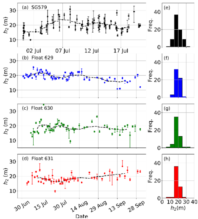
Figure 4. (a–d) Time series of observed h_2 : (a) glider SG579 (black), (b) float 629 (blue), (c) float 630 (green), and (d) float 631 (red). Dashed black lines represent a centred moving average of h_2 values with a window size of 10 data points. (e–h) Histograms of observed h_2 for each glider and floats with the same colour scheme as the time series. The error bars indicate the uncertainty of derived values of h_2 .
