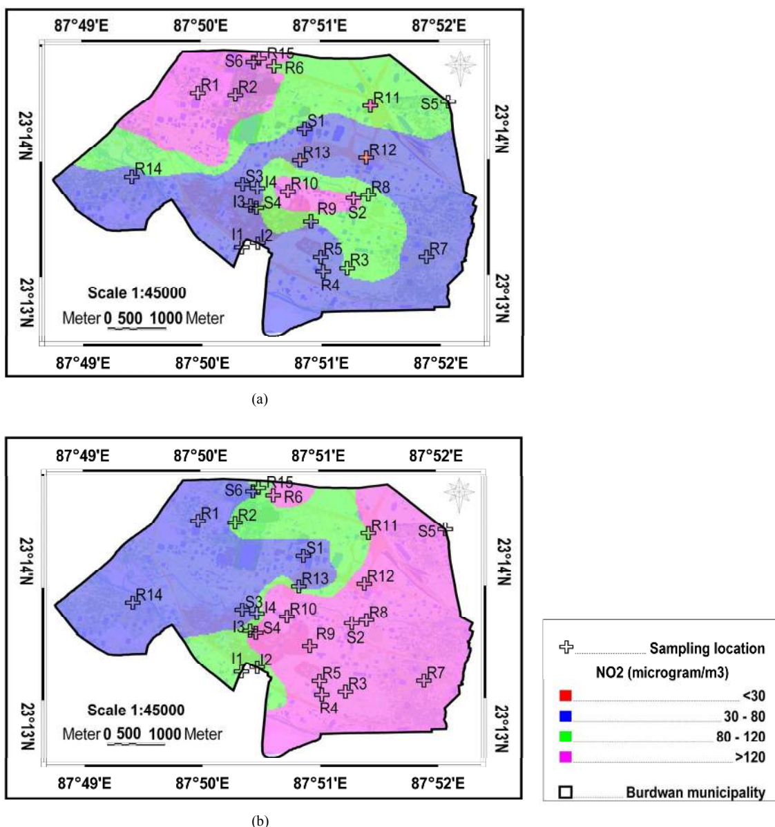
Figure 6. Digital Elevation Model (DEM) on spatio-temporal distribution of \text{NO}_2 over the study area in (a) Pre-monsoon (b) Postmonsoon.
