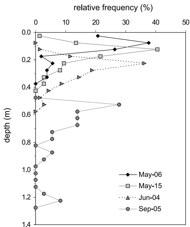
Figure 4. The distribution of frost table depths measured at 40 to 74 points along T1, T2, and T3 on the peat plateau in 2005.
