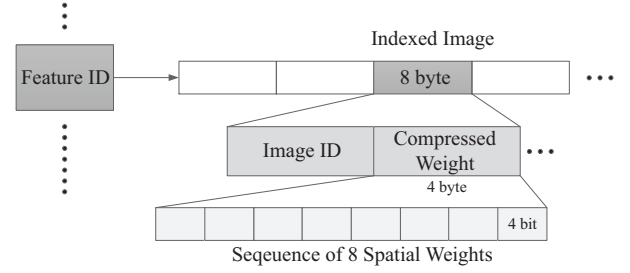
Figure 8. Compressed inverted file structure.
