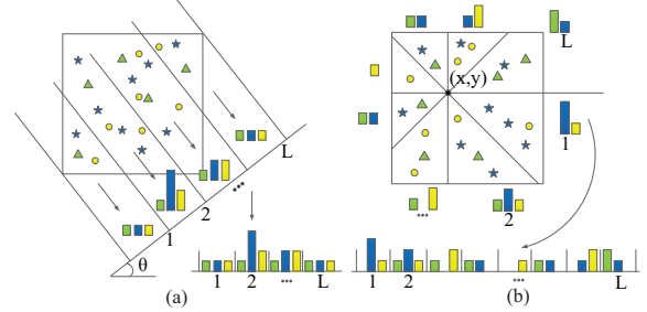
Figure 3. Toy examples of constructing linear and circular ordered bag-of-features. Stars, triangles, and circles represent three kinds of features. (a) Linear projection: all features are projected onto a line with angle \theta and resolution L = 4 , and then the features within each spatial bin are counted. (b) Circular projection: we locate the center at (x, y) and evenly divide the space into L = 8 sectors, and then count features within each sector.
