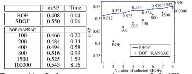
Figure 11. Performance comparison on Oxford5K + Panoramio1M. In the table we provide performances of BOF+RANSAC under our results, where the numbers in the left column represent the number of used top candidates for reranking.
