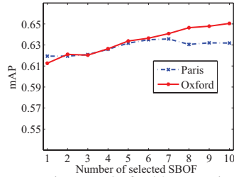
Figure 13. Performance comparison on Oxford5K + Paris.
