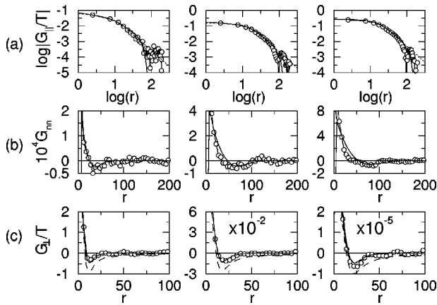
FIG. 2. (a) Longitudinal flow field correlation \log_{10}[G_{\parallel}/T] versus \log_{10} r . (b) Density-density correlation 10^4 G_{nn} versus r ; the same parameters \alpha, \phi, \tau as in Fig. 1 are used for (a) and (b); (c) \mathcal{N}G_{\perp}/T versus r for \phi=0.4 ( I_0 \approx 0.34 ), \alpha=0.6 ( \xi_{\perp}=1.46 , \xi_{\parallel}=3.8 ) at \tau=20, 40 , and 60 (from left to right) with \mathcal{N}=1, 10^{-2} , and 10^{-5} , respectively; in (a) and (c) the solid (dashed) line is the prediction from compressible (incompressible) fluctuating hydrodynamics.
