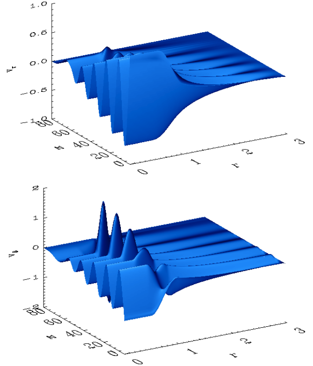
Fig. 3. Snapshot of radial velocity v_r (top) and v_\theta (bottom) as a function of r and z for a kink wave propagating in a cylindrical coronal loop with an inhomogeneous layer ( 0.5 < r \leq 1 ). The velocity components in the core ( r \leq 0.5 ) are damped as the energy is transferred by mode coupling to azimuthal Alfvén oscillations in the inhomogeneous layer.
