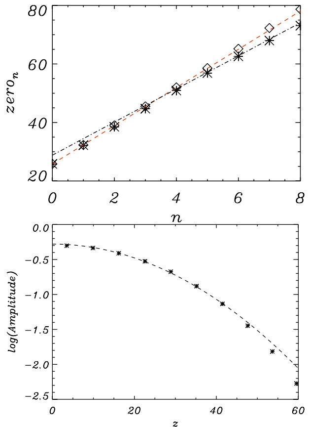
Fig. 5. The top panel shows the location of the zeroes of v_r (crosses) and b_z (diamonds) for the oscillations in Fig. 4. The zeroes for b_z have been shifted to be in phase with those for v_r . The dashed (red) and dot-dashed (black) lines represent the predicted values for the kink mode and Alfvén mode, respectively. The bottom panel shows the natural logarithm of the amplitude of the v_r signal as a function of height. The dashed line indicates Gaussian nature of the spatial damping profile.
