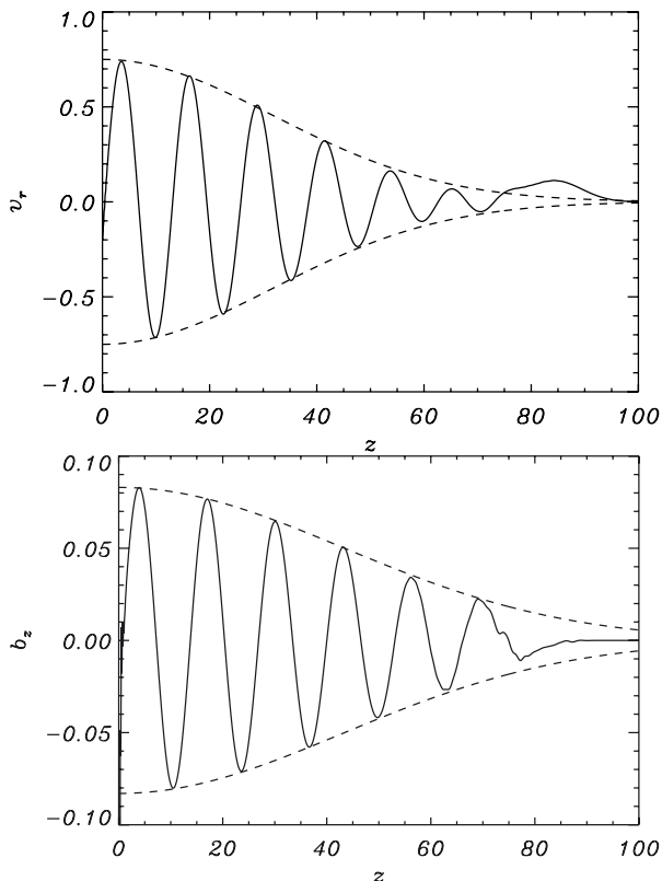
Fig. 4. Radial velocity v_r (top) and longitudinal magnetic field b_z (bottom) as a function of height z at the centre of the inhomogeneous layer. The dashed lines represent a Gaussian envelope of the form given in Eq. (5).
