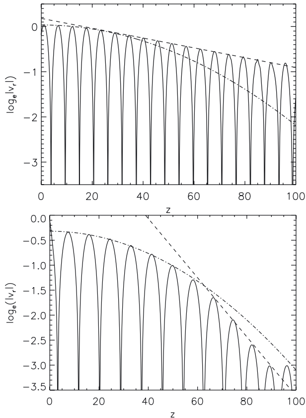
Fig. 6. Logarithmic amplitude of the radial velocity perturbations at the axis of a flux tube for a narrow inhomogeneous layer with l/a = 0.1 , using a driver with a radially discontinuous azimuthal component ( top ) and for a wide inhomogeneous layer l/a = 2/3 , using a smooth driver ( bottom ). The dashed and dot-dashed lines correspond to exponential and Gaussian spatial damping profiles, respectively.
