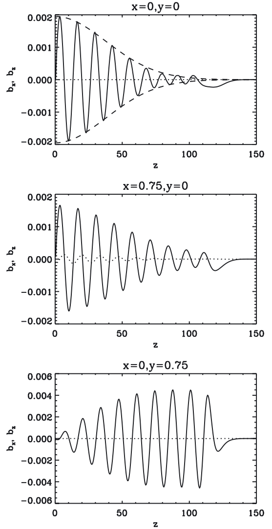
Fig. 1. Magnetic field components as a function of height for a simulation driven with a single harmonic frequency. The solid lines and dotted lines represent b_x and b_z , respectively. The top panel shows the kink mode along the loop axis. The middle panel shows the kink mode inside the inhomogeneous layer. The bottom panel shows the Alfvén mode in the inhomogeneous layer. (Note that b_z has nodes at the (x, y) locations in the top and bottom panels.)
