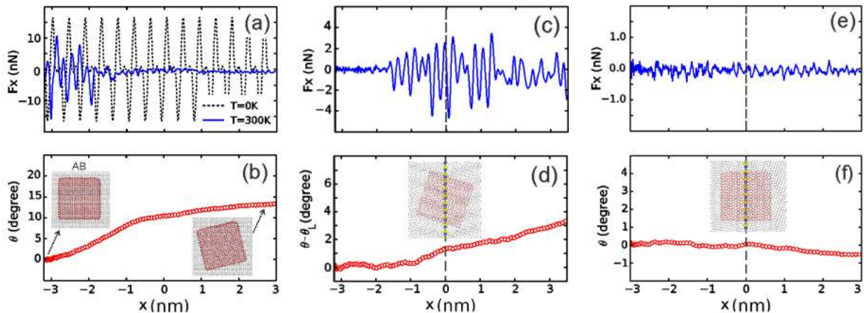
FIG. 3. (color online) The variation of x-component of the total force of a flake moving on (a) pristine graphene, (c,e) a graphene substrate containing a GB line. The variation of corresponding direction \theta of the flake are shown in (b,f) and \theta - \theta_L in (d). The orientation of the flake are shown as insets which have 0^\circ , \theta_L , and 0^\circ in (b), (d), and (f), respectively.
