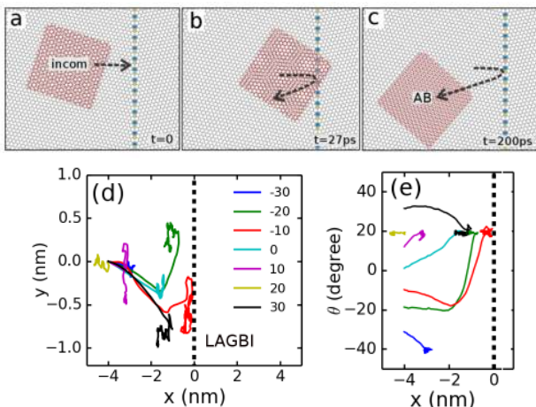
FIG. 4. (color online) Backscattering of a flake moving towards a LAGBI GB when initially it was in an incommensurate state (a,b,c). The path of motion are shown in (d,e) for v_0 = 100 m/s where different colors refer to different initial \theta (given in the inset of (d)).
