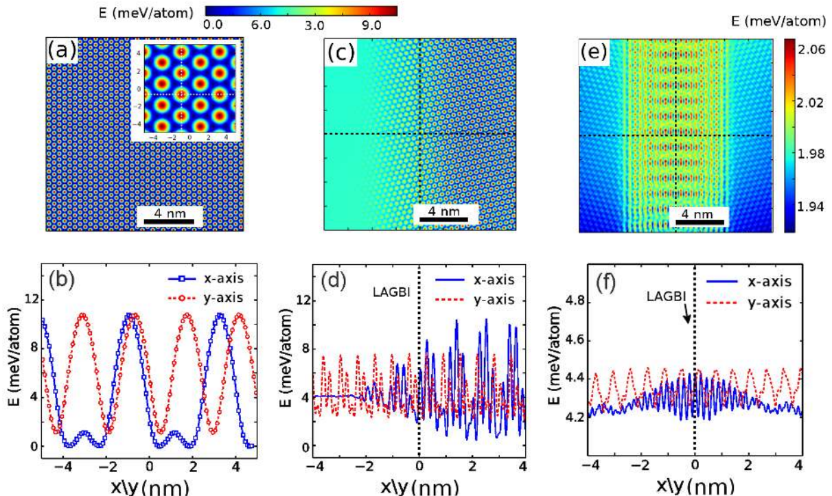
FIG. 2. (color online) (a) The vdW-energy landscape resulting from the vdW-energy stored between the graphene flake above a perfect graphene substrate at z=0.34 nm and (b) two corresponding cross sections along the armchair and zig-zag directions indicated by dashed lines in the inset of (a). In (c) ((e)), we show the energy landscape of the flake rotated with \theta = \theta_L(0^\circ) scanned inside the box \oplus ( \otimes ) as shown in Fig. 1 and the corresponding cross sections along the dashed lines are shown in (d) ((f)). Energy reference is chosen to be E_{AB}=0 .
