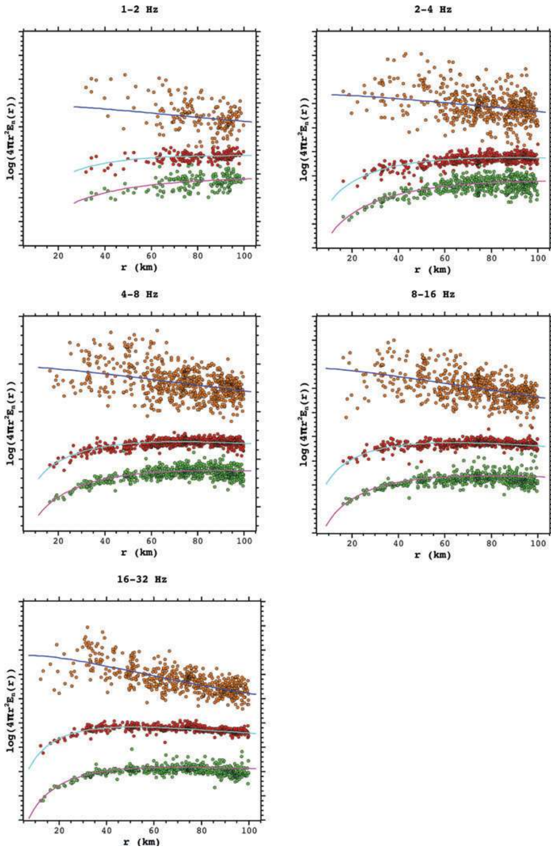
Figure 3. Example of MLTWA. Data and the best-fitting curves for the Hi-net station N.YMDH located in the northeast Japan for all the frequency bands. Orange, red and green points correspond to the first, second and third window, respectively. The continuous lines corresponds to the fitting carried out by using a synthetic model. The location of the station N.YMDH is indicated in Fig. 1(a) by means of red triangle.
