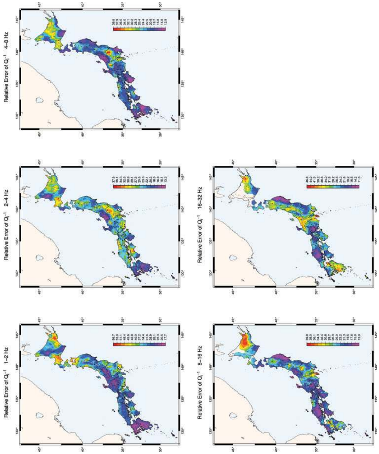
Figure B1. Estimation of the errors computed by using the variance-covariance matrix of each fitting for Q_1^{-1} for each frequency band.
