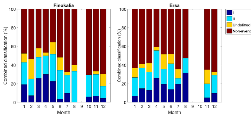
Figure 3. Monthly classification of the measurement days into event (I and II), undefined, and non-event categories in Finokalia and Ersa.
