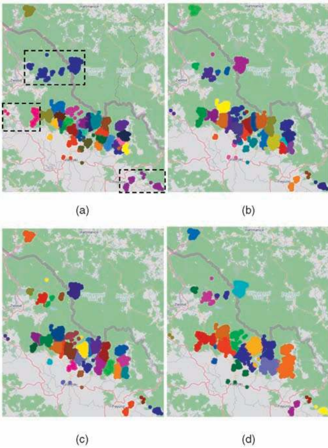
Fig. 7. (a) The characteristic points extracted from the trajectories of the roe deer have been clustered by the “simple k-means” method. (b) The same points have been grouped by Algorithm 2; \text{MaxRadius} = 3,000 m. (c) The groups resulting from Algorithm 2 have been optimized using Algorithm 3. (d) The points have been grouped by Algorithms 2 and 3 with \text{MaxRadius} = 5,000 m. In all cases, the groups are represented by colors of the circles representing the points.
