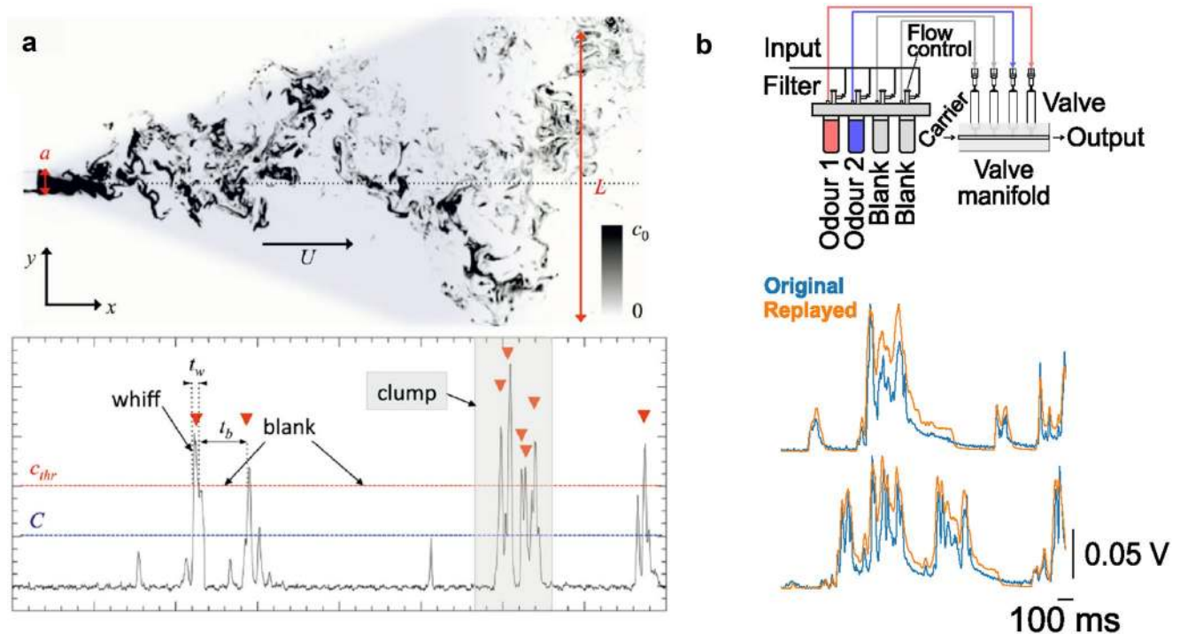
Fig. 1 Structure and reproduction of complex odour plumes. a Top: Two-dimensional section of a turbulent odour plume highlighting its chaotic distribution in water. Bottom: Recording of the odour concentration fluctuation over time at a given point in space (from Celani et al. 2014). b Top: Schematic of a multi-channel high band-
