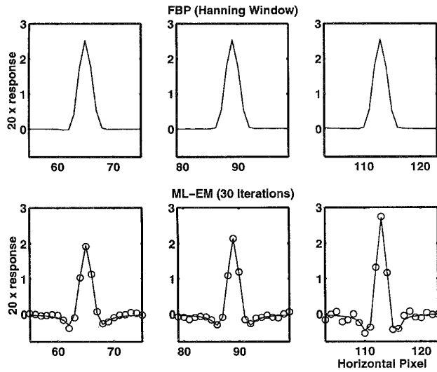
Fig. 1. Horizontal profiles through the local impulse response functions of FBP with a Hanning window (top) and of the ML-EM algorithm at 30 iterations (bottom), for three pixels located along the horizontal midline of an elliptical object. Solid line: computed using the linearized approximation (10). Circles: computed using the unbiased estimator (6) from M = 2000 realizations.
