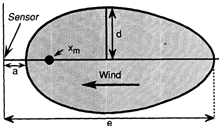
Fig. 4. Dimensions of a turbulent source area isopleth. x_m : maximum source location (upwind distance of the surface element with the maximal influence on a given sensor); a : downwind edge, e : upwind edge and d : lateral half-dimension of the source area.
