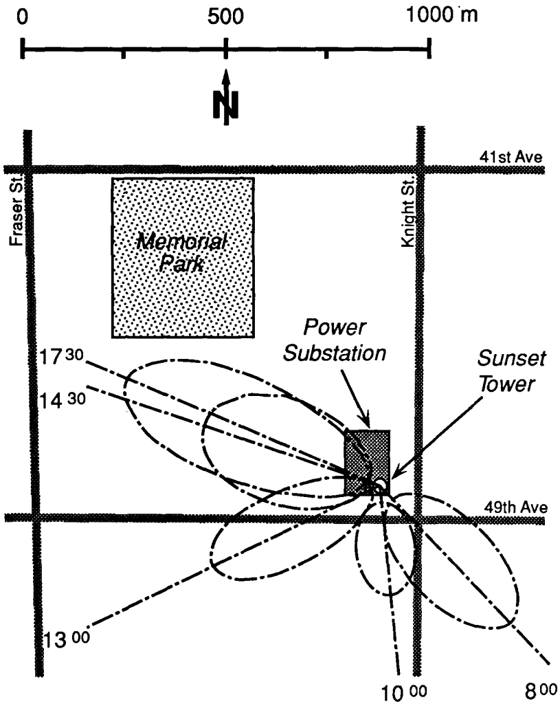
Fig. 7. The evolution of the turbulent source area during YD 86/231 for the Sunset tower site. The alignment of the 0.5-level isopleths varies with wind direction, and their dimensions are dependent on atmospheric stability and lateral turbulence intensity. The variable thermal properties within the source area over time provide a link between the temporal and spatial variability of turbulent sensible heat flux.
