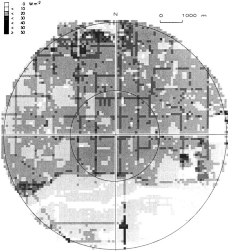
Fig. 10. Map of anthropogenic heat flux for 9:00 L.A.T. on YD 87/22. Hectare grid centered on the Sunset site. The inner circle has a radius of 2 km.
