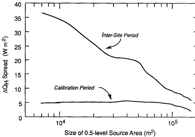
Fig. 9. Dependence of the spatial variability of sensible heat flux ( \Delta Q_H Spread) on the size of the source area. With increasing source area the measurements of sensible heat flux are representative of a larger area and their spatial variability is reduced. This effect is absent when two instruments mounted on the same tower are compared during a calibration period.
