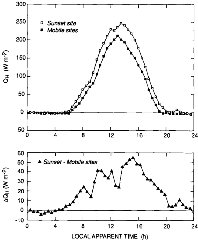
Fig. 8. Comparison of the mean daily variations of turbulent sensible heat flux between the Sunset site and the composite mobile sites. The differences between the two ( \Delta Q_H ) is plotted in the lower part on an expanded scale.
