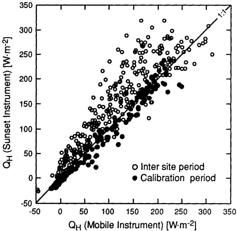
Fig. 6. Synchronous observations of hourly sensible heat flux at the Sunset site and the composite of five mobile sites (empty circles); comparison of the two instrument sets used (filled circles).
