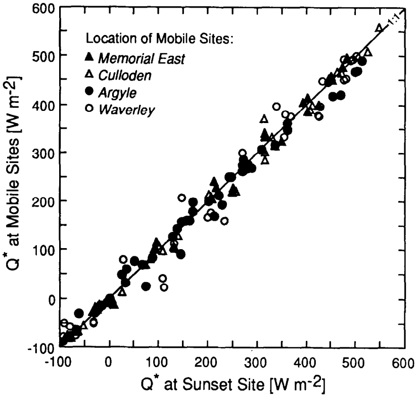
Fig. 5. Synchronous observations of hourly net radiation at the Sunset site and the composite of four mobile sites.
