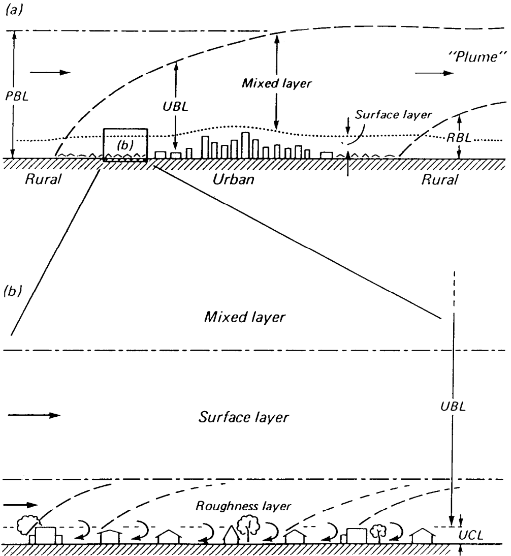
Fig. 1. Conceptual arrangement of boundary-layer structure over a city; (a) at the meso-scale ( \sim 10^1 km); (b) at the local scale ( \sim 10^{-1} km) (after Oke, 1984).
