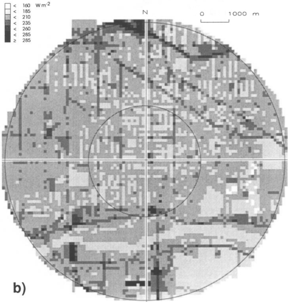
Fig. 11. Map of storage heat flux; (a) 8:00 L.A.T.; (b) 12:00 L.A.T. (ensemble of all days modelled). Hectare grid centered on the Sunset site. The inner circle has a radius of 2 km.
