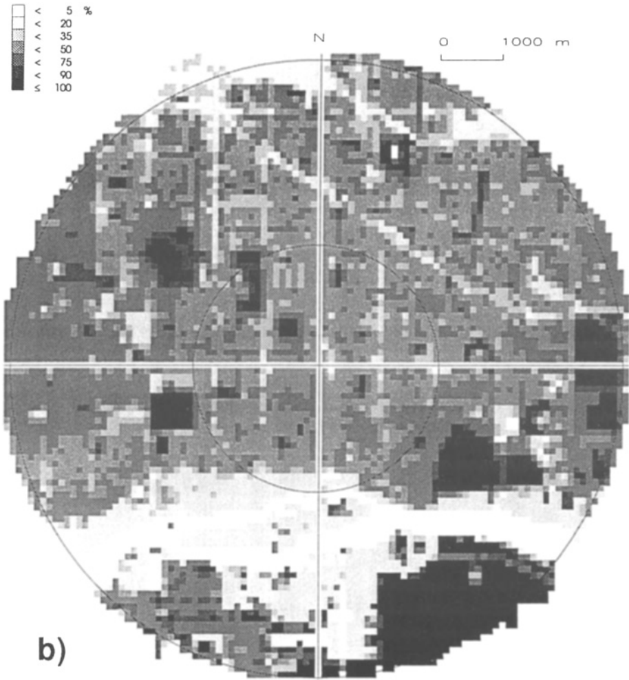
Fig. 3. Maps of surface type from the data base on a hectare grid, centered on the Sunset site. The inner circle has a radius of 2 km. (a) paved surface; (b) total vegetation (in % of the entire grid-cell).
