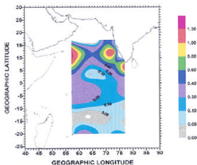
Figure 3. Spatial variation of \tau_p at 500 nm during the IFP-99 cruise. Each colour corresponds to a given range of \tau_p as identified by the vertical bar by the side. The ground station \tau_p data from Trivandrum during the cruise and from Goa prior to the cruise are also incorporated.
