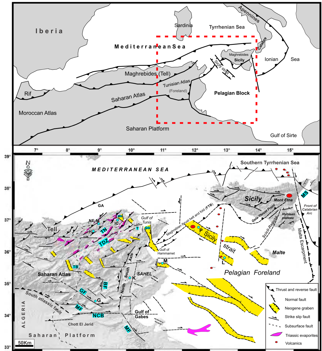
Figure 1. Tectonic sketch of Tunisia and surrounding regions with location of the study area. TN: Tellain nappes (Maghrebides), TDZ: Triassic diapirs zone, MG: Mateur graben, GA: Galite Island, NE-M: Nefza-Mogodos, Hairech, Ichkeul, GG: Grombalia graben, K: Kairouan, MF: Metlaoui fault, BF: Bir Hfey fault, GF: Gafsa fault, G: Gafsa region, T: Tunis, TB: Tebessa, M: Monastir region, P: Pantelleria Island, L: Linosa, NCB: northern Chott fault, MF: Medenine fault system, and MS: Messinian Strait.
