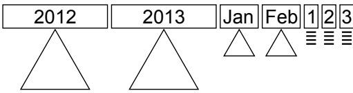
Figure 5: Spatio-temporal index
