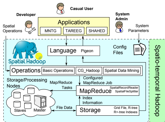
Figure 1: Overview of SpatialHadoop
