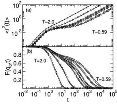
FIG. 2. (a) Mean-square displacement for several state points studied. (b) Coherent intermediate scattering function F(q_0, t) calculated at q_0 \approx 7.5 for several state points studied.
