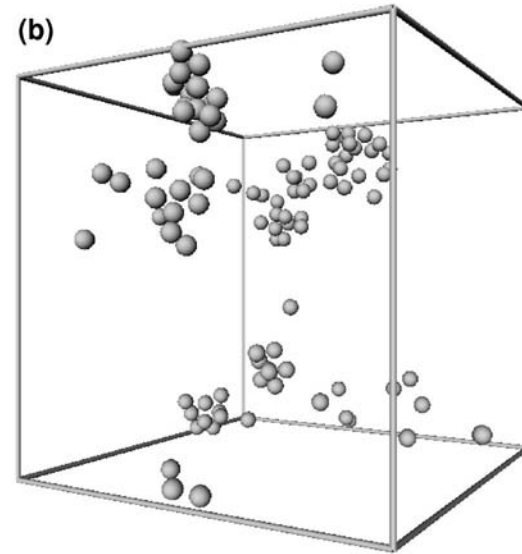
FIG. 17. (a) Snapshot of localized particles at t=t_4^{\max} and T=0.60 . The fraction is \langle Q_S/N \rangle = 0.244 . (b) Snapshot of localized particles at t=0.03t_4^{\max} and T=0.60 . \langle Q_S/N \rangle = 0.01 .
