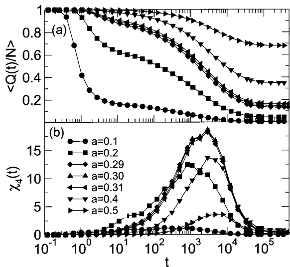
FIG. 22. (a) Q(t) as a function of a at T=0.59 for a=0.1, 0.2, 0.29, 0.3, 0.31, 0.4, and 0.5 . (b) \chi_4(t) as a function of a . The position of the peak in \chi_4(t) for a=0.29, a=0.30, and a=0.31 is the same. The amplitude of \chi_4(t) is strongest for a=0.3 .
