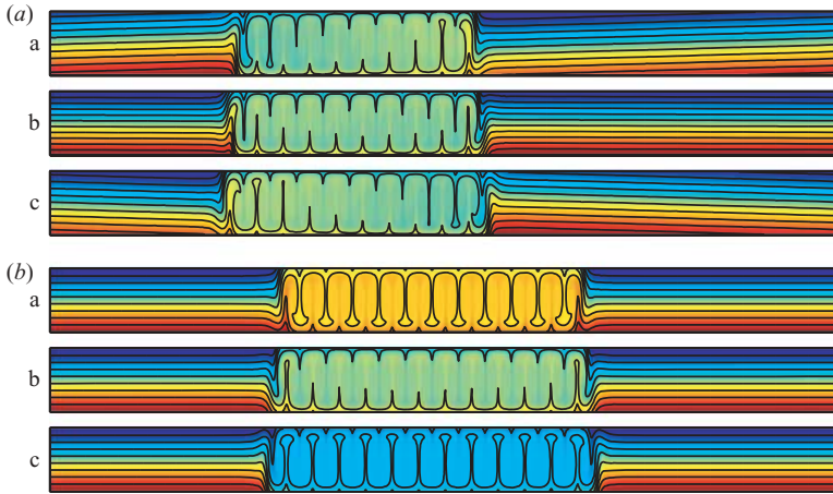
FIGURE 5. Convecton profiles on (a) the odd-parity branch, and (b) the even-parity branch at the turning points indicated in figure 4(a, b) in terms of contours of constant C . Each wavelength contains a pair of rolls.
