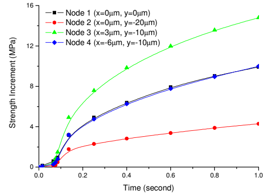
Fig. 13 Temporal evolution for four discrete material points of strength increment by geometrically necessary dislocation density
