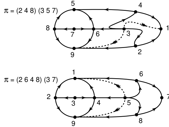
Fig. 2.3. C^0 orbit equivalent Sturm attractors \mathcal{A}_f with nonconjugate permutations \pi_f . Note how the attractors differ in the geometry of the fast unstable manifolds, indicated by double arrows.
