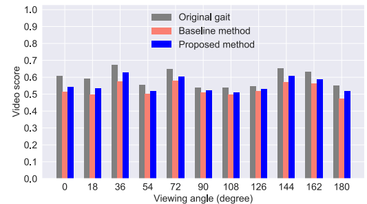
Figure 14: Video score.
