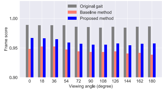
Figure 13: Frame score.
