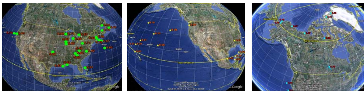
Fig. 1 Spiral locations for INTEX-NA (left), INTEX-B (middle), and ARCTAS (right) and associated integrated column values in E21molec/cm 2 .
