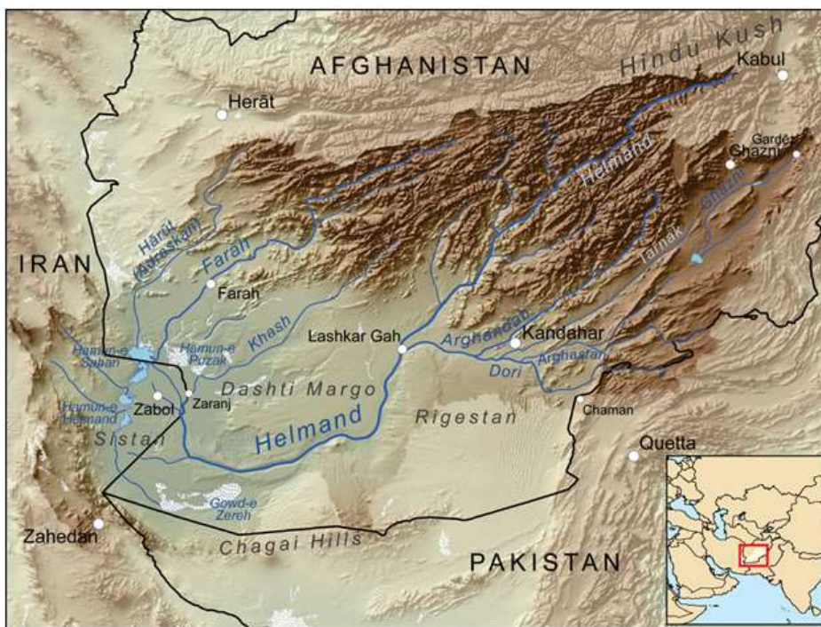
Figure 1: Topographic map of Sistan region and Hamoun Basin. The bold color in the map defines the Helmand drainage basin that fed Hamoun lakes complex. [source: http://en.wikipedia.org/wiki/Sistan_Basin ]
