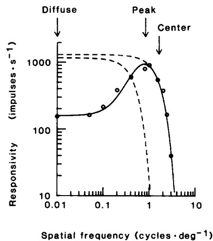
FIGURE 1. Method for choosing stimulus spatial frequencies. The circles show responsivities for an on-center X cell (13X8) as a function of the spatial frequency of gratings drifting at 2 Hz. (Responsivity is the amplitude of the fundamental Fourier component of the impulse rate divided by the stimulus contrast.) The continuous curve is the best fit of the Gaussian center-surround model described in the Methods. The dashed curves show the responsivities of the center and surround components of the model. The "diffuse" stimulus was a grating with a spatial frequency of 0.01 cycles·deg -1 , the "peak" stimulus had a spatial frequency that maximized responsivity, and the "center" had a spatial frequency that was chosen to give a responsivity between two and four times less than that with the peak stimulus. The mean luminance of the screen was 340 cd·m -2 , and the cat had a 4-mm-diam artificial pupil.
