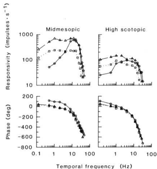
FIGURE 6. X cell spatiotemporal frequency response at lower mean levels of retinal illumination. Spatiotemporal frequency responses for an on-center X cell (11X5) are given for a midmesopic (mean luminance, 2.8 \text{ cd} \cdot \text{m}^{-2} ) and a high scotopic (mean luminance, 0.021 \text{ cd} \cdot \text{m}^{-2} ) level of light adaptation. Responsivity and phase are shown as a function of temporal frequency for diffuse ( 0.01 \text{ cycles} \cdot \text{deg}^{-1} , circles), peak ( 1.22 \text{ cycles} \cdot \text{deg}^{-1} , triangles), and center ( 2.0 \text{ cycles} \cdot \text{deg}^{-1} , squares) stimuli.
