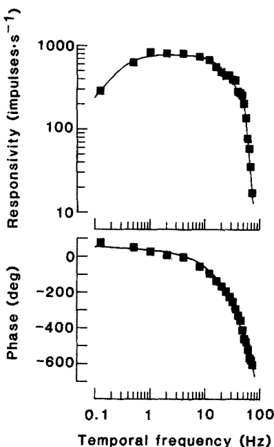
FIGURE 13. Fit of a model with six first-order low-pass filters, one second-order filter, a transitional lead, and a time delay to the temporal photopic frequency response measured with the peak stimulus for the unit (13X8) that was featured in Figs. 1, 8, and 10. For this particular cell, the corner frequencies for the six low-pass filters were at 46 Hz and the corner frequency for the second-order filter was at 53 Hz. The second-order filter had a damping constant of 0.17. The parameters g and \tau of the transitional lead were 9 and 4 s, respectively. The time delay was 15 ms and the overall gain was 800 \text{ impulses} \cdot \text{s}^{-1} .
